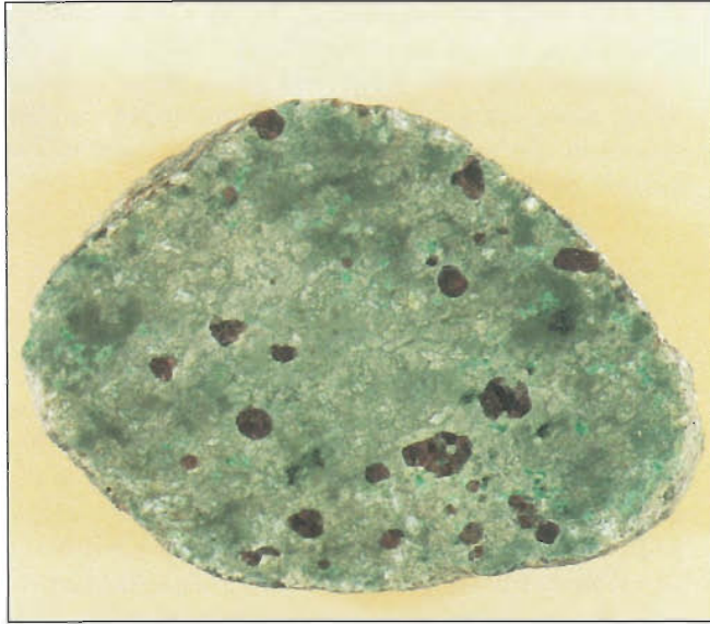
Plate 1a. Garnet peridotite nodule collected from the Schaffer group of kimberlites in the Colorado-Wyoming State Line district. The peridotite contains rounded, reddish, pyrope garnet porphyroblasts with green chromian diopside (a clinopyroxene) in a serpentinized matrix. Much of the serpentine forms replacements after olivine.
