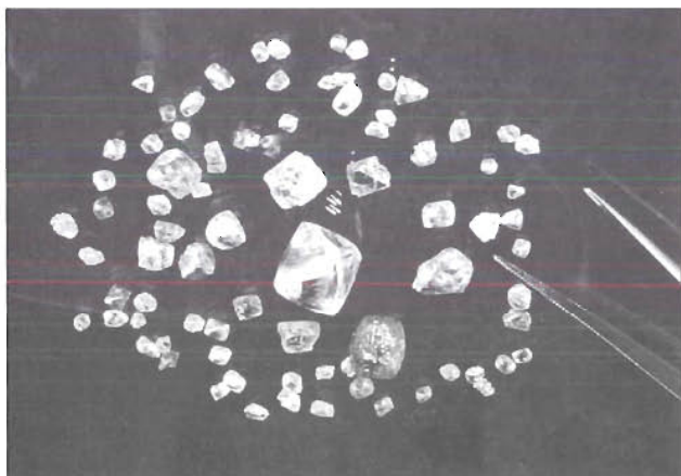
Figure 13. A sampling of several gem-quality diamonds recovered from the Kelsey Lake diamond mine. The largest stone in the center weighed 14.2 carats. Photograph courtesy of Redaurum Ltd. and Howard Coopersmith.
