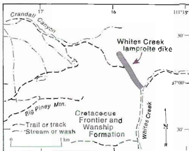
Figure 43. Location map of the Whites Creek lamproite dikes, Utah (after Mitchell and Bergman, 1991).
