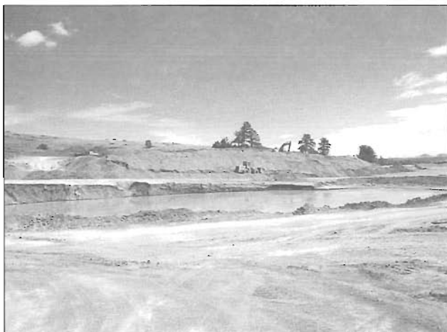
Figure 12. The kimberlite at Kelsey Lake is weathered and very soft; as a result, the material is scraped and no blasting is necessary.
