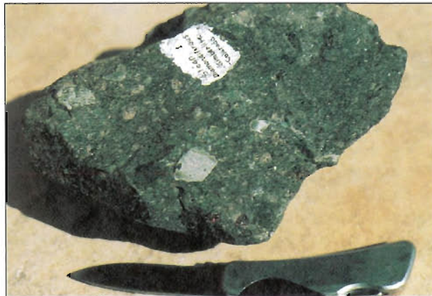
Plate 1b. Hand specimen of diatreme facies kimberlite from the Sloan 1 intrusive, Colorado-Wyoming State Line district. Clasts of country rock including a reddish pyrope megacryst are seen in the breccia.
