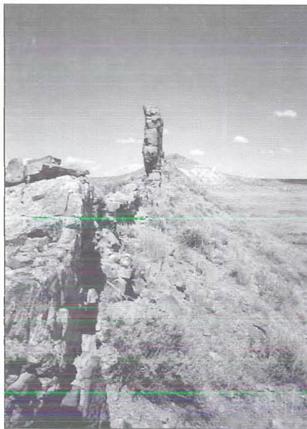
Figure 35. A portion of the dike complex at Smoky Butte.
