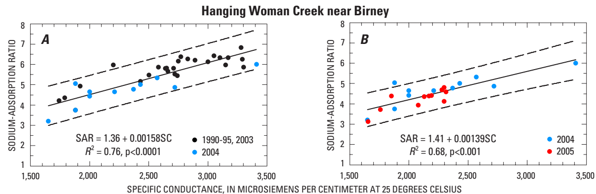
Figure 20. Relation of specific conductance (SC) and sodium-adsorption ratio (SAR) for water-quality samples collected at Hanging Woman Creek near Birney, Montana: A , Relation used to estimate SAR for the 2004 irrigation season and based on data collected March 1990 through June 2004; B , Relation used to estimate SAR for the 2005 irrigation season and based on data collected October 2003 through July 2005. Dashed lines indicate 95-percent prediction interval.
