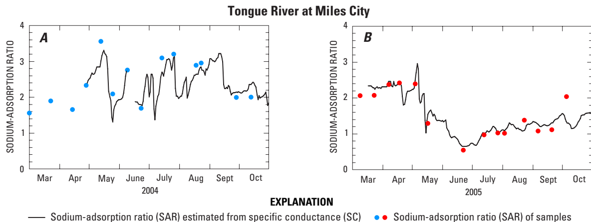
Figure 15. Sodium-adsorption ratio (SAR) determined from water-quality samples and estimated from specific conductance (SC) for Tongue River at Miles City, Montana, using relations shown in figure 14: A , 2004 irrigation season; B , 2005 irrigation season.
