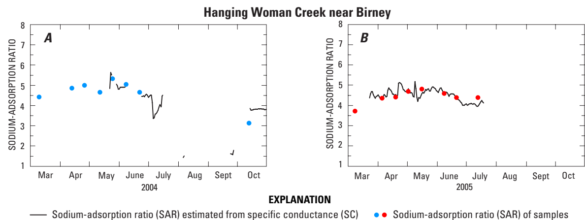
Figure 21. Sodium-adsorption ratio (SAR) determined from water-quality samples and estimated from specific conductance (SC) for Hanging Woman Creek near Birney, Montana, using relations shown in figure 20: A , 2004 irrigation season; B , 2005 irrigation season.
