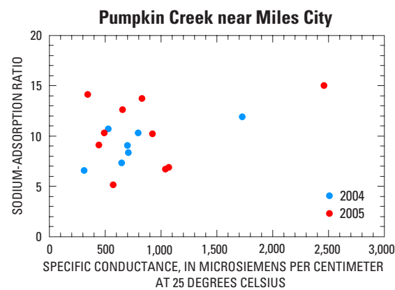
Figure 24. Specific conductance (SC) and sodium-adsorption ratio (SAR) for water-quality samples collected March 2004 through October 2005 at Pumpkin Creek near Miles City, Montana (estimated SAR values are not available for this site for 2004–06).
