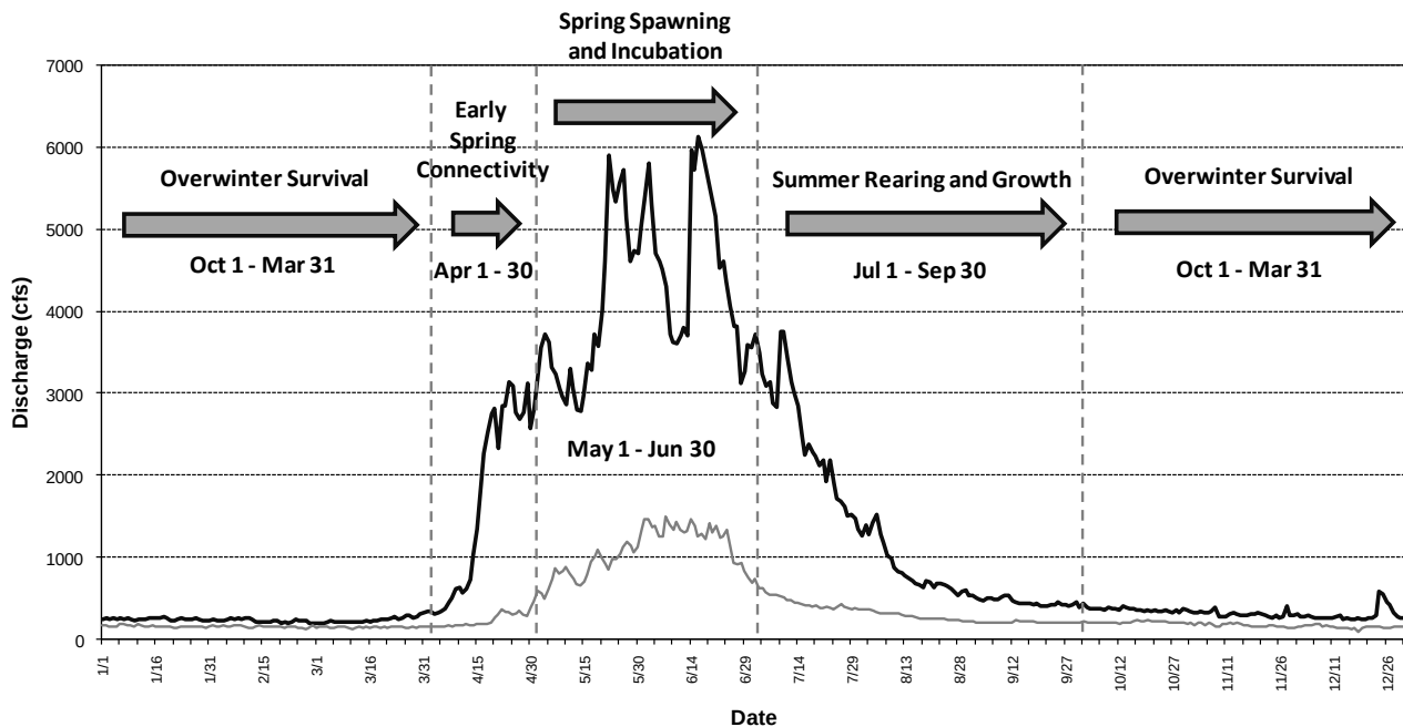
FIGURE 6. Minimum and maximum daily historical discharge values in the Hoback River and critical time periods for SRC. Data are from USGS gage 13019500 on the Hoback River (1944–1958).
