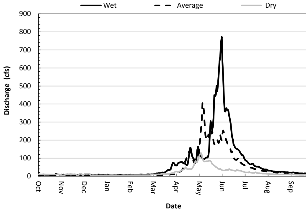
FIGURE 7. Simulated annual hydrographs for randomly selected wet (1984), average (1989), and dry (1987) water years at the Dell Creek instream flow segment (HabiTech 2009).
