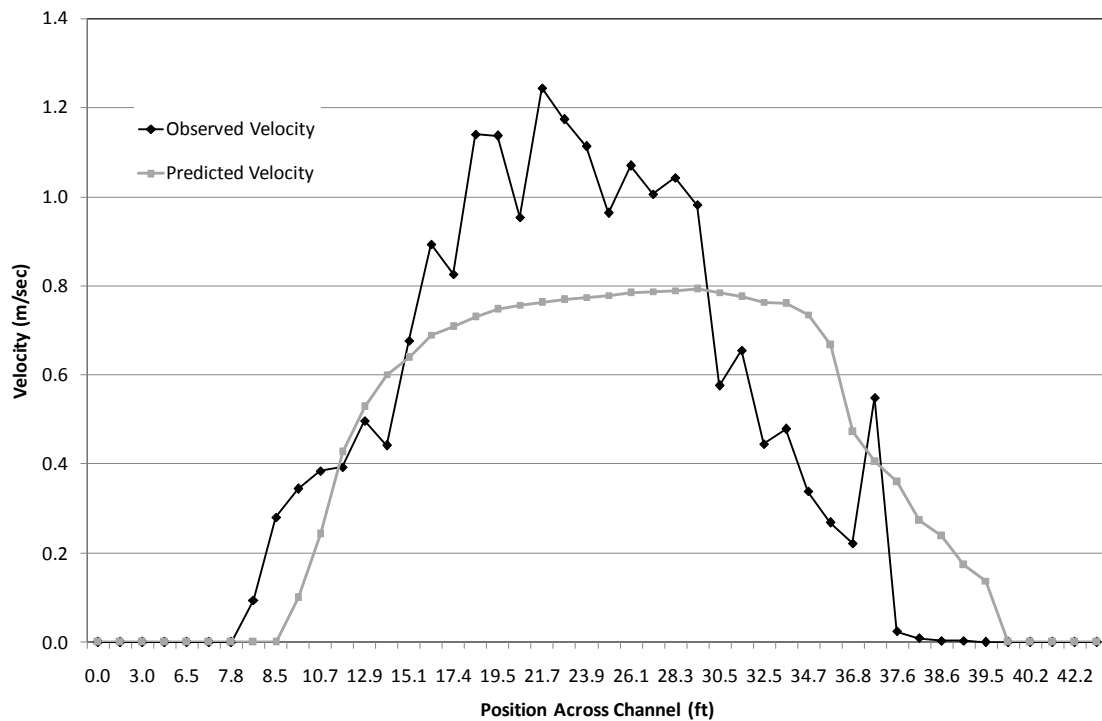
FIGURE 9. Final model-predicted and observed velocities at 95 cfs along the upstream cross-section in the Dell Creek study site.
