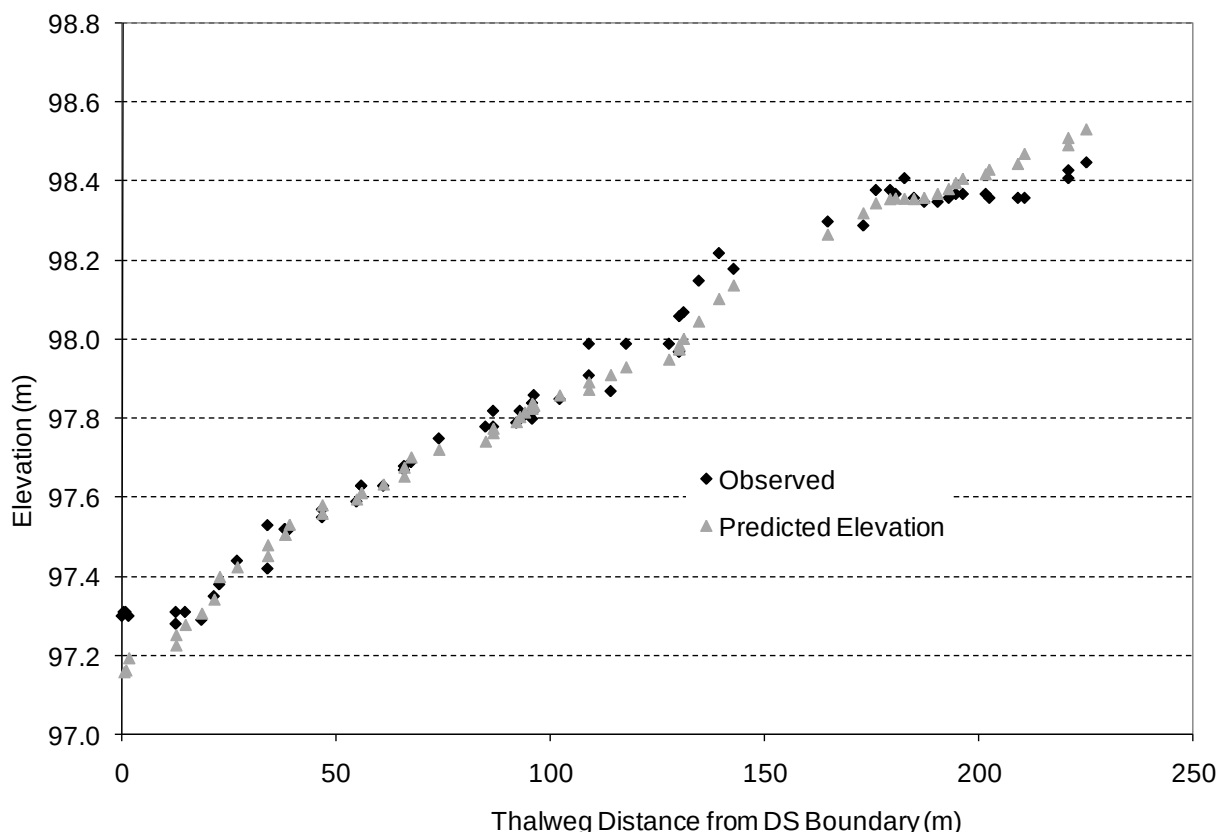
FIGURE 8. Final model-predicted and observed water surface elevations at 95 cfs along the left bank in the Dell Creek study site.
