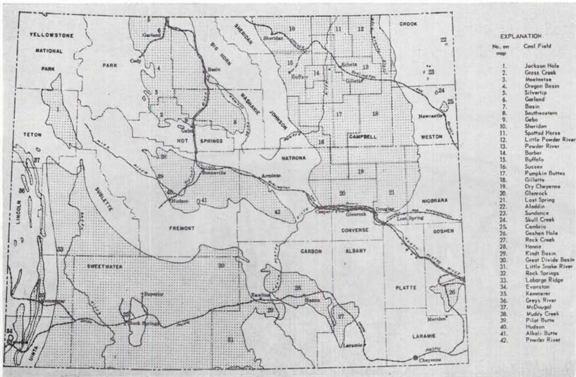
Fig. 3. Coal fields of Wyoming (After Berryhill, et al., 1950 U. S. Geol. Surv. Circular 81.
