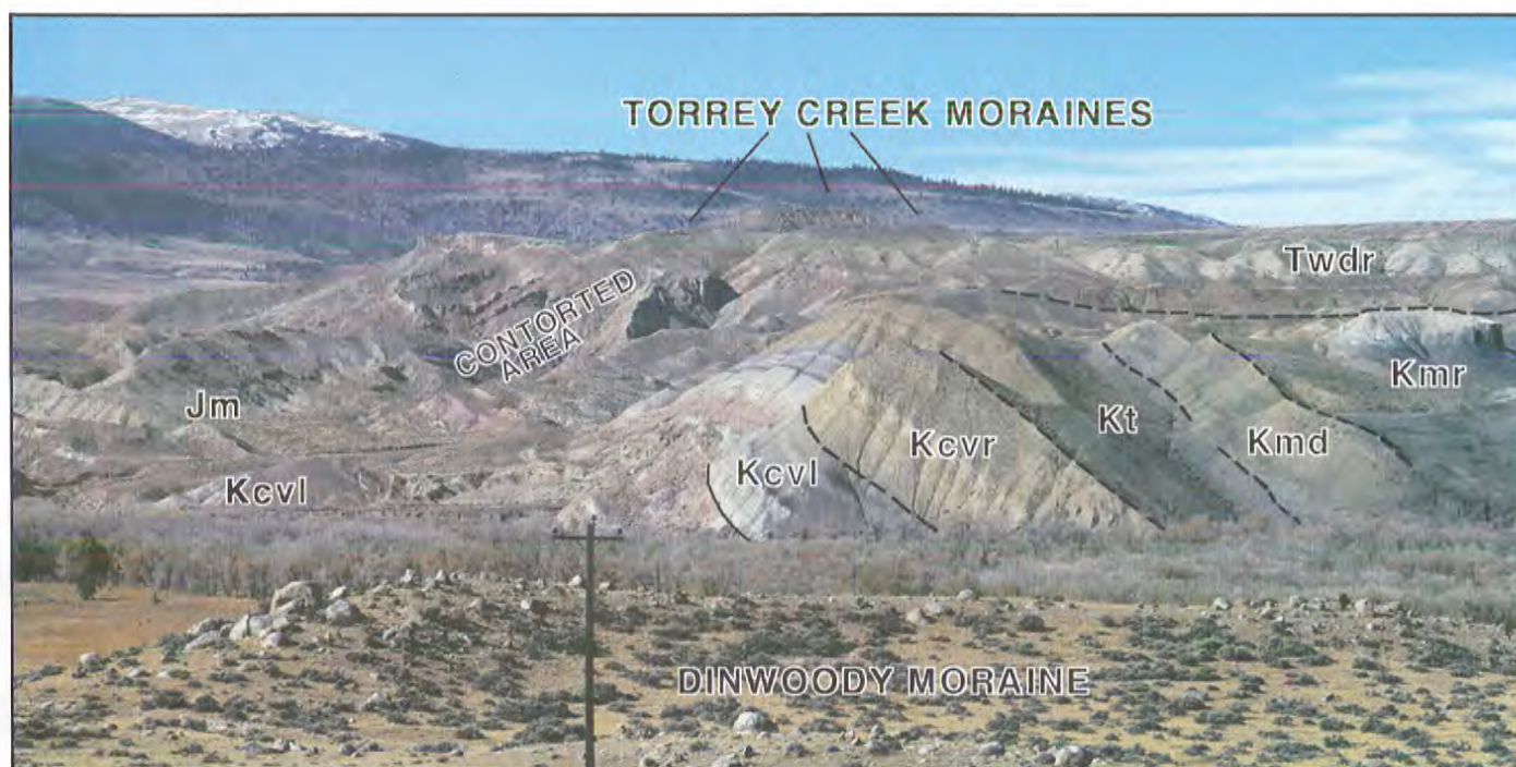
Figure 20. View northwest from Stop 7. Wind River Range are on left skyline. Indicated are: Jm - Morrison Formation (Jurassic); Kcvi - lilac claystone zone in Cloverly Formation, Kcvi - rusty beds member in Cloverly Formation, Kt - Thermopolis Shale, Kmd - Muddy Sandstone Member of Thermopolis Shale, and Kmr - Mowry Shale, all of Cretaceous age; and Twdr - Wind River Formation of Eocene age. Photograph by J.D. Love, October 25, 1979.
