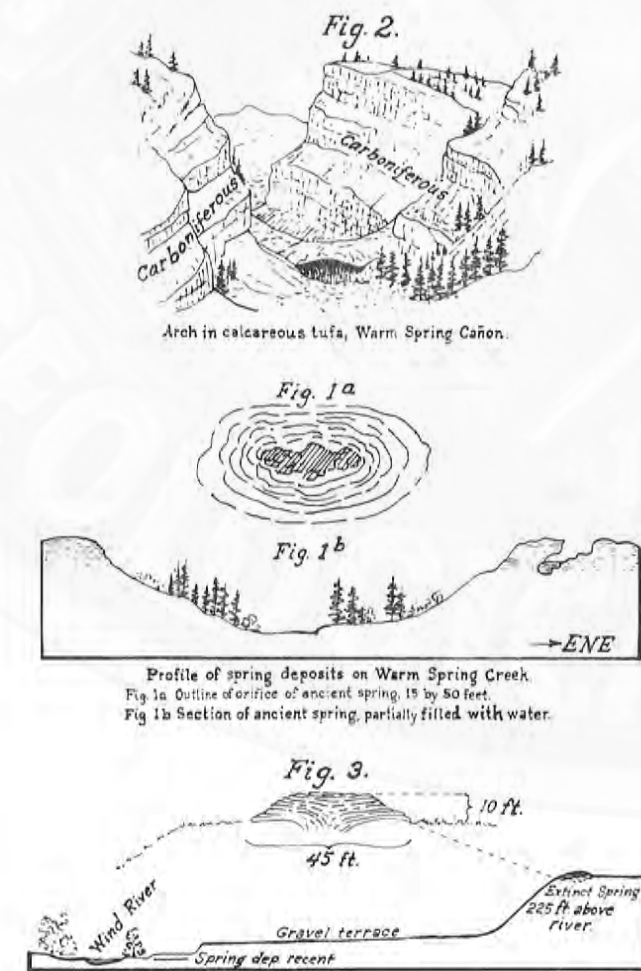
Figure 15. Sketches of travertine deposits and associated strata, Warm Spring Creek Canyon. Reproduced from Plate XLIX by St. John, in Hayden (1883).
