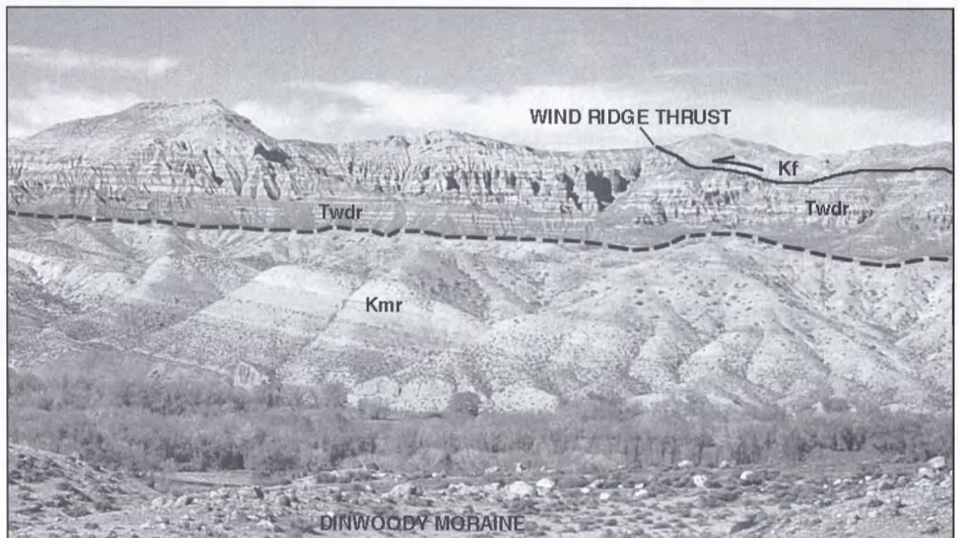
Figure 22. Close-up view of a part of Figure 21. Indicated are: Kmr - Mowry Shale (Cretaceous); unconformably overlain by Twdr - Wind River Formation (Eocene). Thrust fault on the Wind River Formation has Kf - Frontier Formation (Cretaceous) on the upper thrust plate. Photograph by J.D. Love, October 25, 1979.
