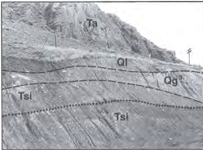
Figure 4. Lacustrine sequence of the Shooting Iron Formation (Tsl), folded into gentle anticline delineated by main fossil zone (dotted line); porphyritic andesite (Ta); post-Bull Lake loess (Ql); and outwash of Bull Lake Glaciation (Qg 3 ). Modified from Love and Taylor (1962).
