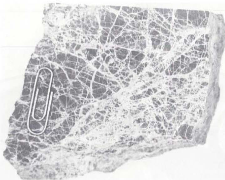
A. Photograph of cataclastically deformed sample of Bighorn Dolomite. Sample taken less than 1 centimeter from a thrust plane contact. Note intense fragmentation along a locus of shear in lower right corner. Paper clip for scale is three cm long.
