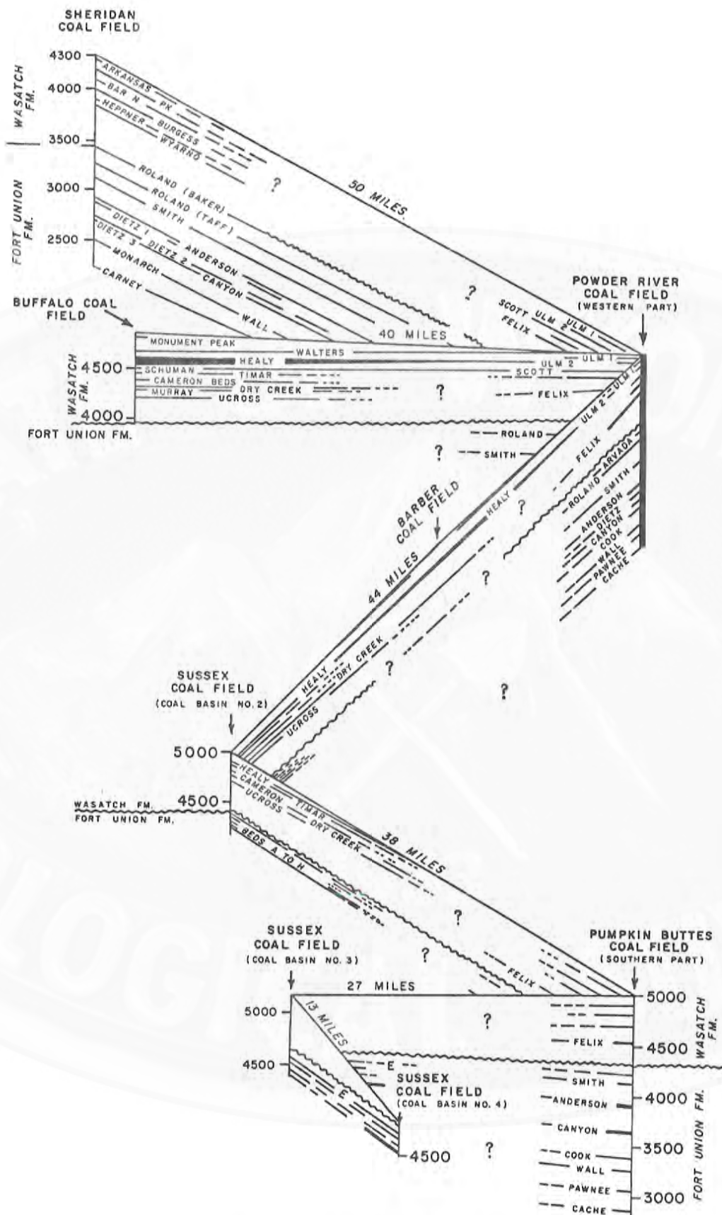
Figure 6. Correlation of Coal Beds in the Powder River Coal Basin.
