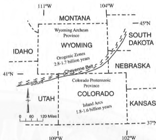
Figure 8. Regional setting of the Precambrian glaciation that followed planation creating a continental platform in Wyoming.
