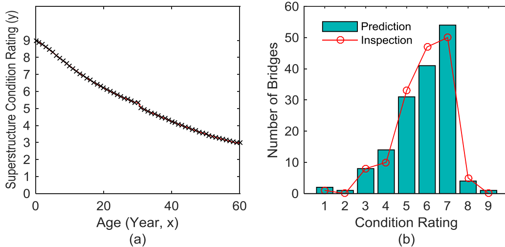
Figure 58. Graph. (a) Deterioration model and (b) comparison between prediction and inspection result in terms of number of bridges versus condition rating for rest bridges
