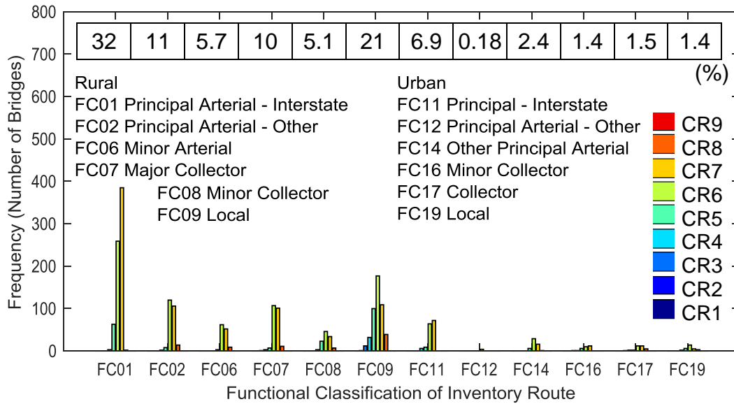
Figure 26. Chart. Distribution for Functional Classification of Inventory Route
