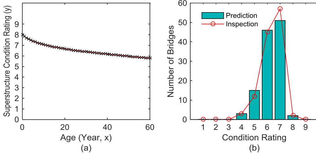
Figure 83. Graph. (a) Deterioration model and (b) comparison between prediction and inspection result in terms of number of bridges versus condition rating for WSO (None) and DL0 (Other/Unknown) bridges
