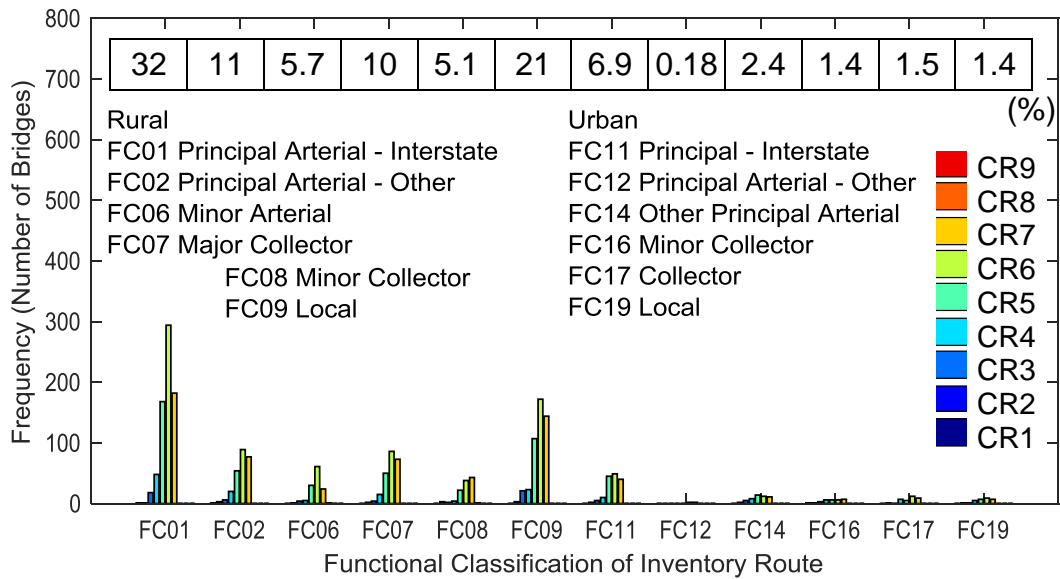
Figure 15. Chart. Distribution for Functional Classification of Inventory Route
