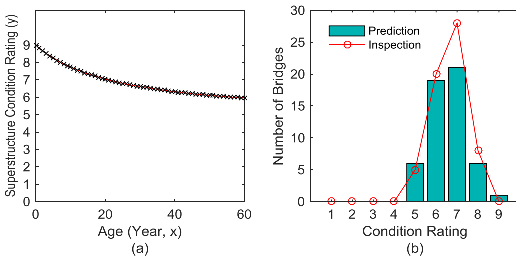
Figure 68. Graph. (a) Deterioration model and (b) comparison between prediction and inspection result in terms of number of bridges versus condition rating for DST1 (Concrete Cast-in-Place) and BRW1 (0 – 5 m, 0 ft – 16.4 ft), BRW5 (20 m, 65.5 ft) bridges
