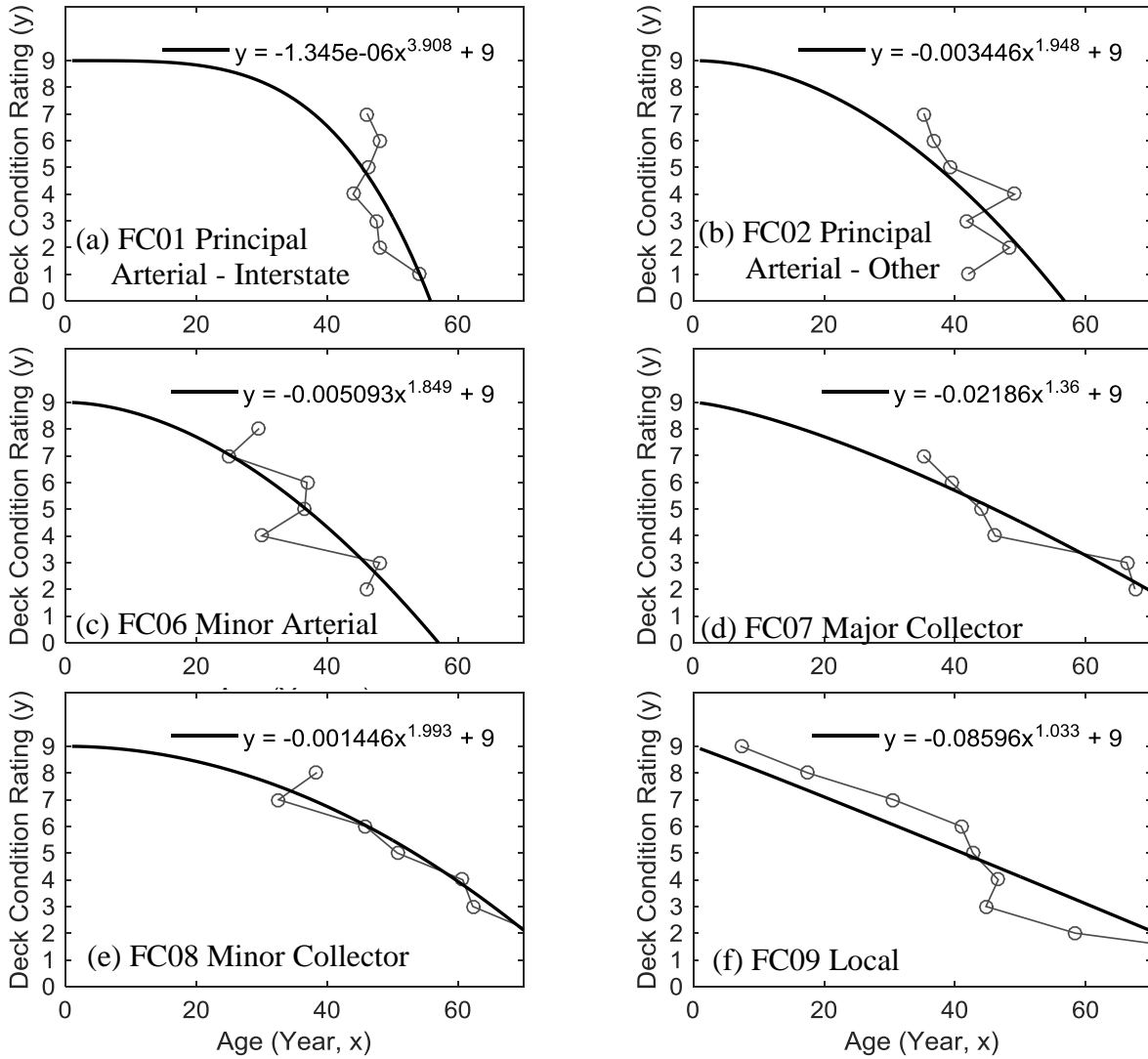
Figure 16. Graph. Deterioration models for Functional Classification of Inventory Route belonging to the rural category
