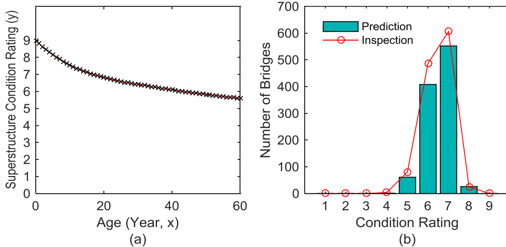
Figure 61. Graph. (a) Deterioration model and (b) comparison between prediction and inspection result in terms of number of bridges versus condition rating for DST1 (Concrete Cast-in-Place) and BRW3 (10 – 15 m, 32.8 – 49.2 ft) bridges
