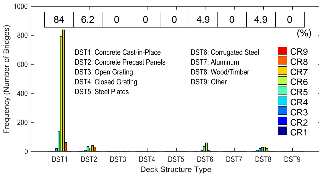
Figure 22. Chart. Distribution for Deck Structure Type
