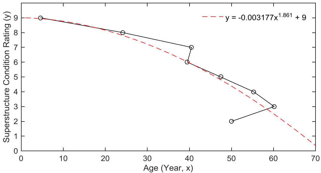
Figure 21. Graph. General deterministic deterioration model for superstructure elements
