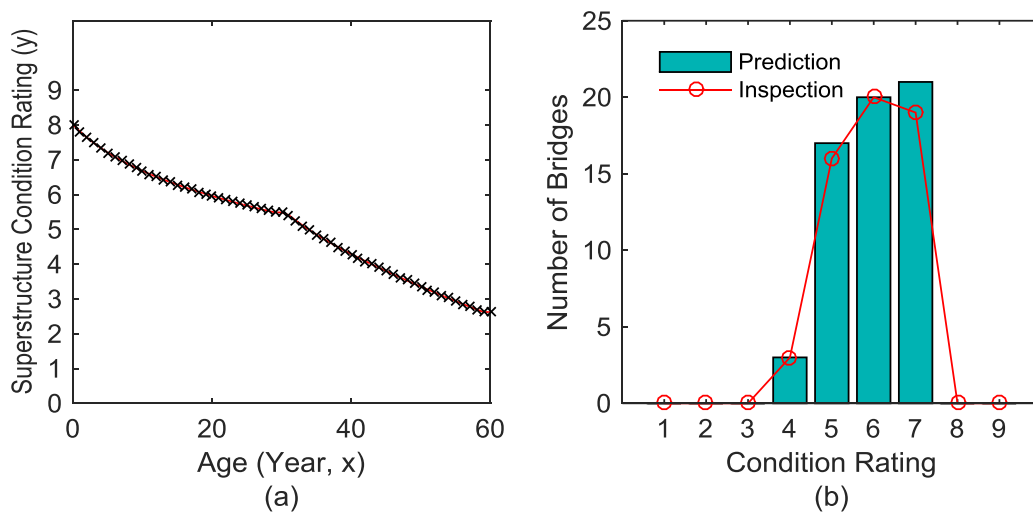
Figure 74. Graph. (a) Deterioration model and (b) comparison between prediction and inspection result in terms of number of bridges versus condition rating for WS6 (Bituminous) and DL2 (M 13.5) bridges
