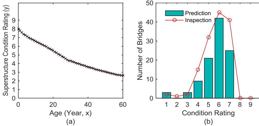
Figure 50. Graph. (a) Deterioration model and (b) comparison between prediction and inspection result in terms of number of bridges versus condition rating for WS3 (Latex Concrete/Similar) and SL2 (50 – 100 m) bridges
