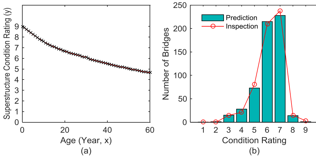
Figure 51. Graph. (a) Deterioration model and (b) comparison between prediction and inspection result in terms of number of bridges versus condition rating for WS6 (Bituminous) and SL1 (0 – 50 m) bridges
