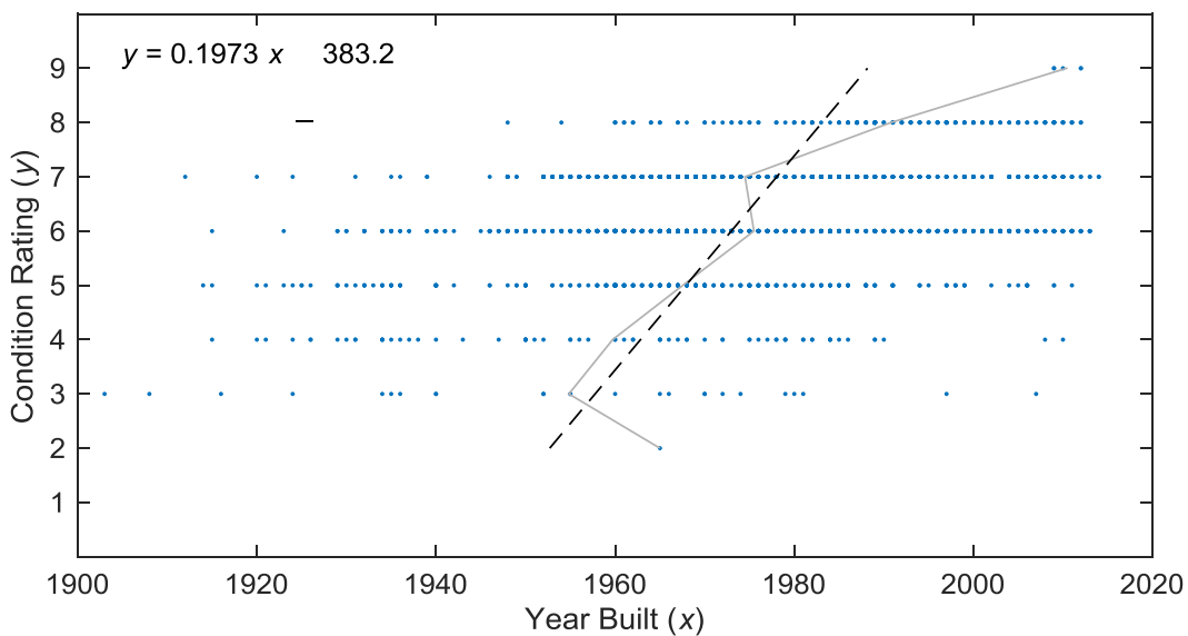
Figure 20. Graph. Condition rating versus year built for bridge superstructure at year 2014
