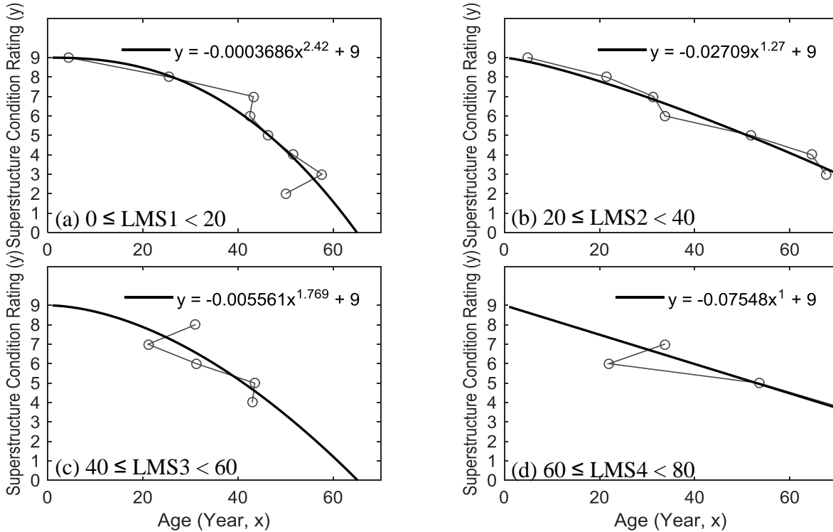
Figure 30. Graph. Deterioration models for Length of Maximum Span
