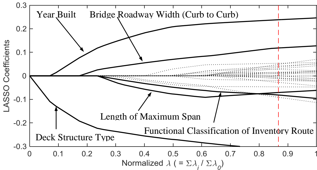
Figure 7. Graph. Solution path for superstructure condition ratings by LASSO
