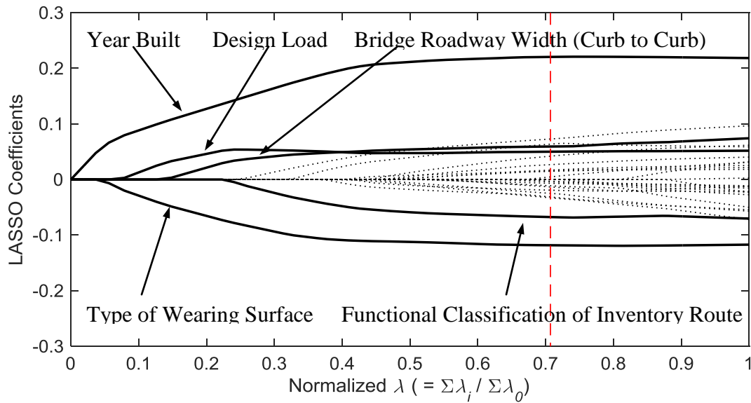
Figure 8. Graph. Solution path for substructure condition ratings by LASSO
