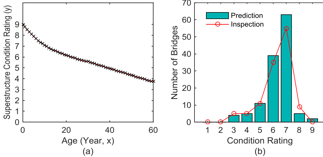
Figure 88. Graph. (a) Deterioration model and (b) comparison between prediction and inspection result in terms of number of bridges versus condition rating for rest bridges
