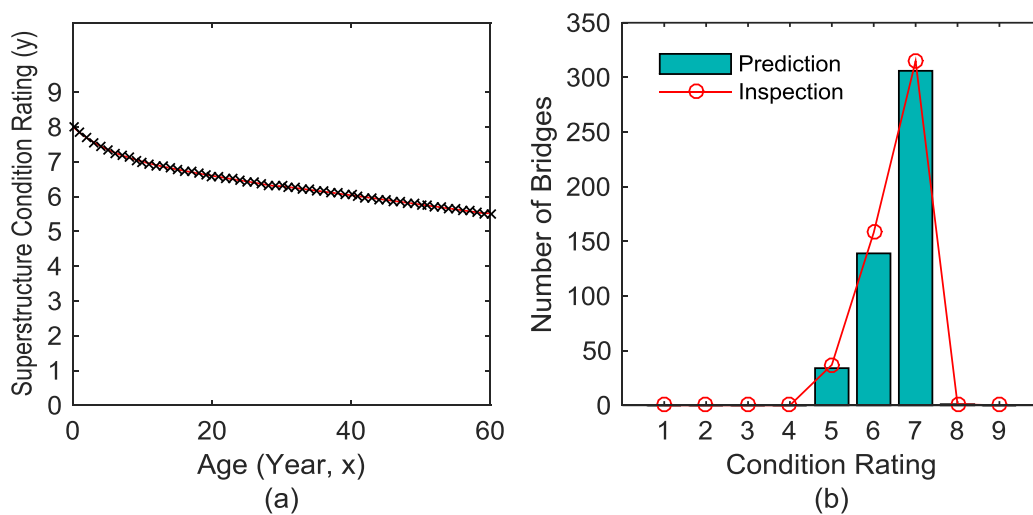
Figure 80. Graph. (a) Deterioration model and (b) comparison between prediction and inspection result in terms of number of bridges versus condition rating for WS0 (None) and DL5 (MS 18) bridges
