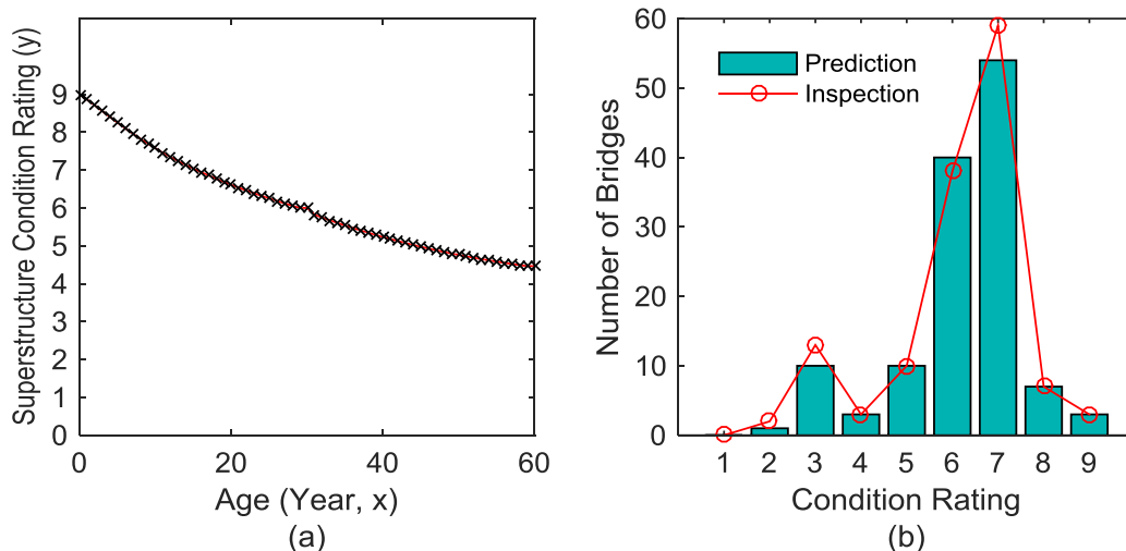
Figure 53 (a) Deterioration model and (b) comparison between prediction and inspection result in terms of number of bridges versus condition rating for WS8 (Gravel) and SL1 (0 – 50 m) bridges
