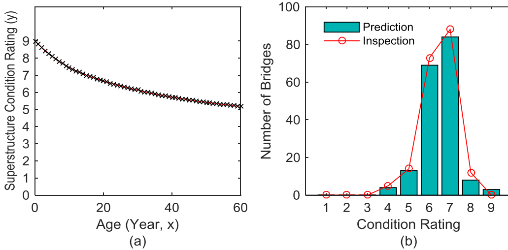
Figure 75. Graph. (a) Deterioration model and (b) comparison between prediction and inspection result in terms of number of bridges versus condition rating for WS6 (Bituminous) and DL5 (MS 18) bridges
