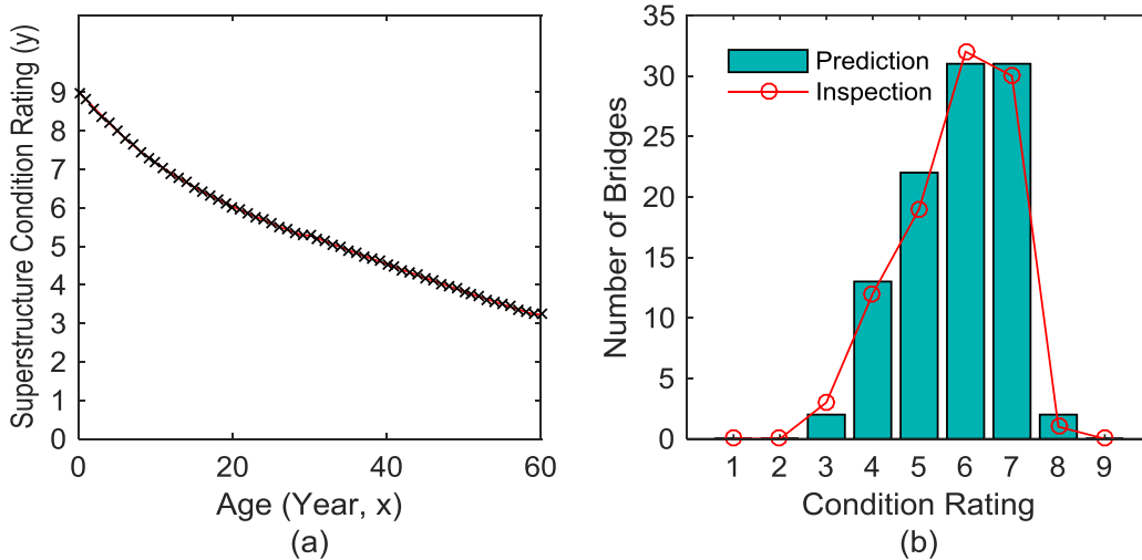
Figure 67. Graph. (a) Deterioration model and (b) comparison between prediction and inspection result in terms of number of bridges versus condition rating for DST8 (Wood/Timber) and BRW2 (5 – 10 m, 16.4 ft – 32.8 ft)bridges
