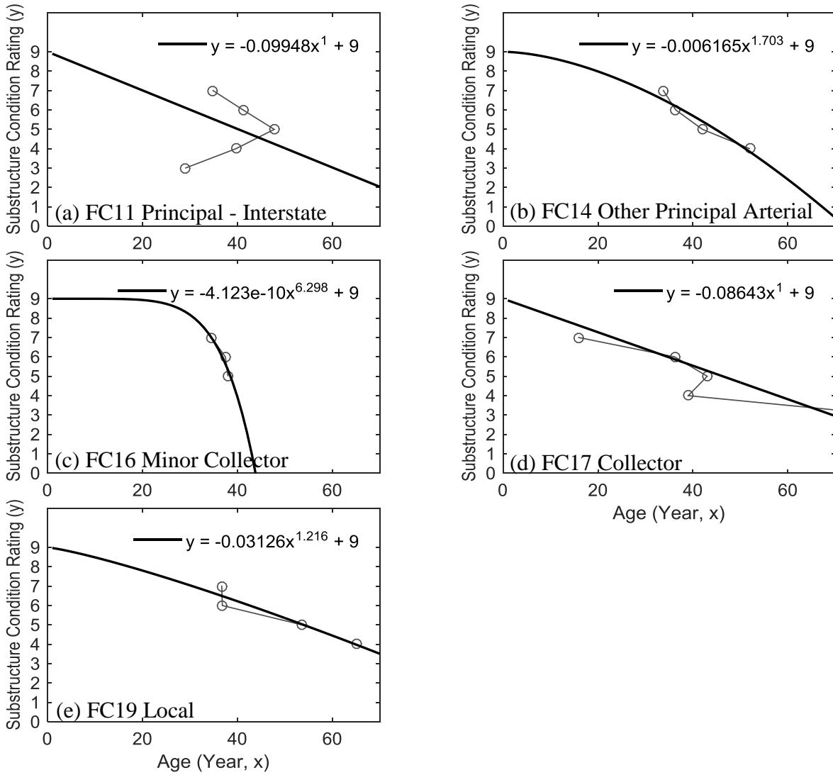
Figure 41. Graph. Deterioration models for Functional Classification of Inventory Route
