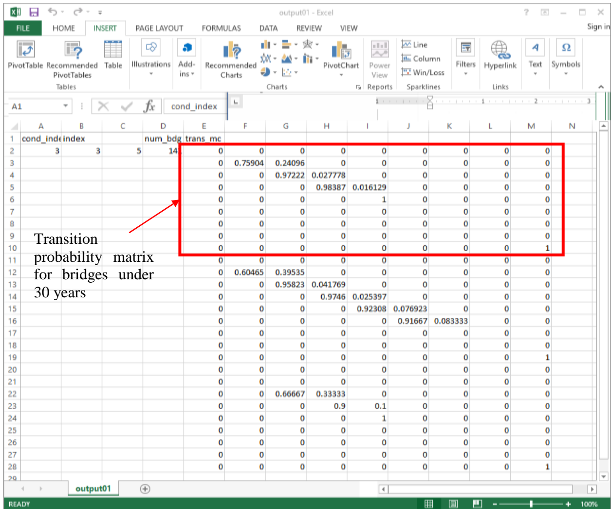
Figure 92. Screen Capture. Output file example
