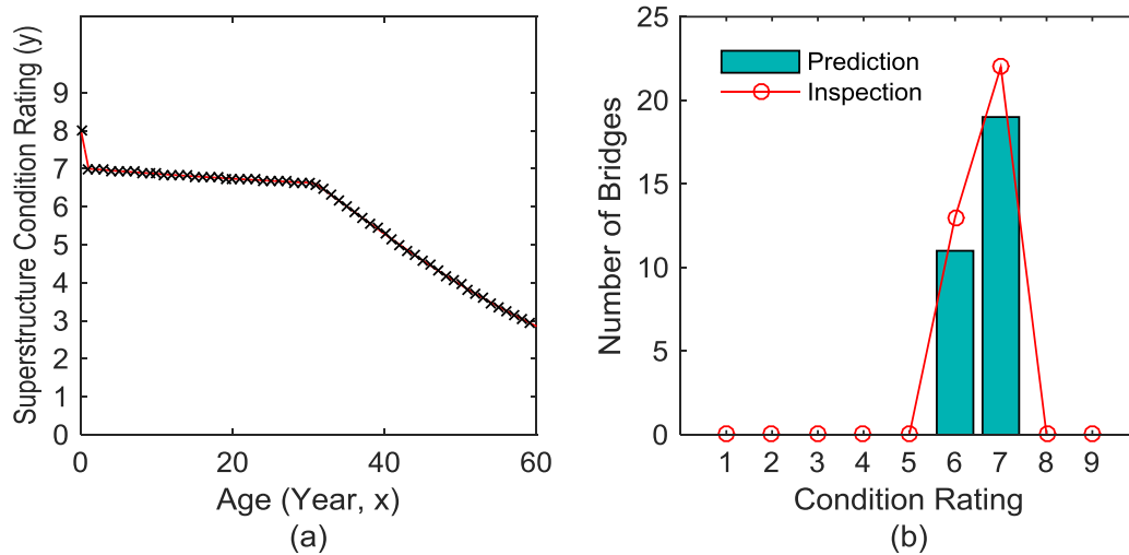
Figure 84. Graph. (a) Deterioration model and (b) comparison between prediction and inspection result in terms of number of bridges versus condition rating for WS5 (Epoxy Overlay) and DL0 – DL9 (all) bridges
