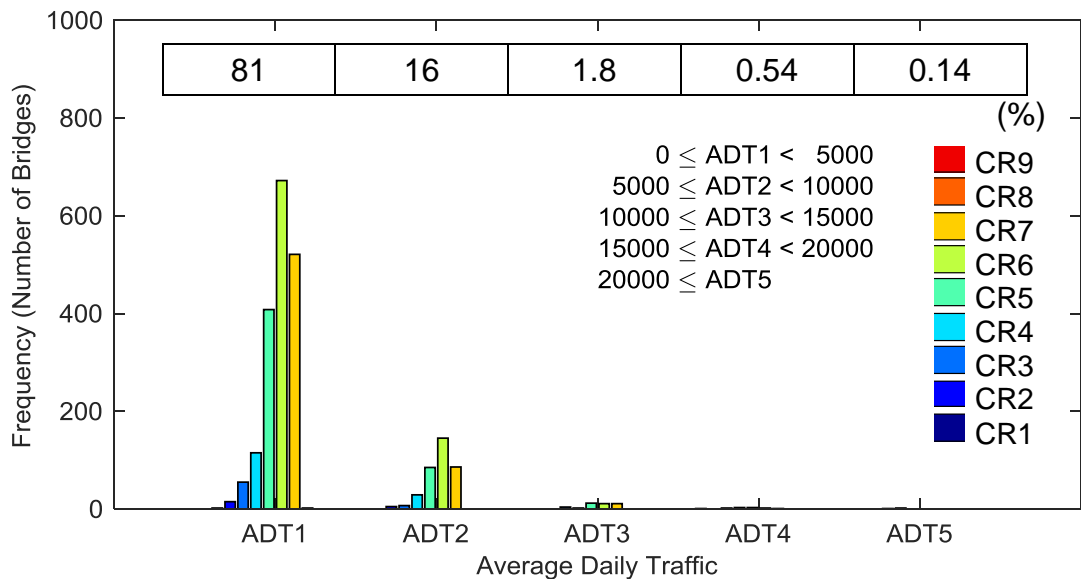
Figure 18. Chart. Distribution for Average Daily Traffic
