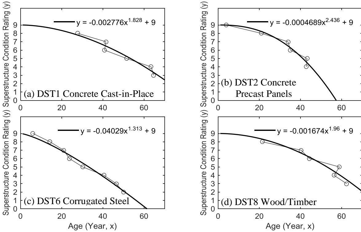
Figure 23. Graph. Deterioration models for Deck Structure Type
