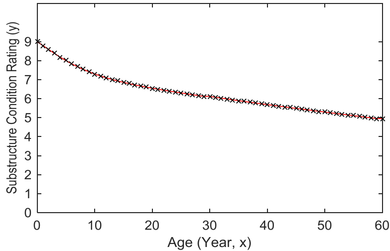
Figure 71. Graph. Deterioration model for substructure element
