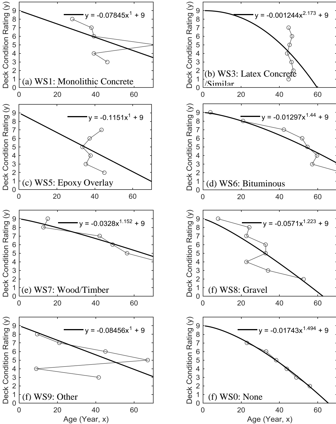
Figure 12. Graph. Deterioration models for Type of Wearing Surface
