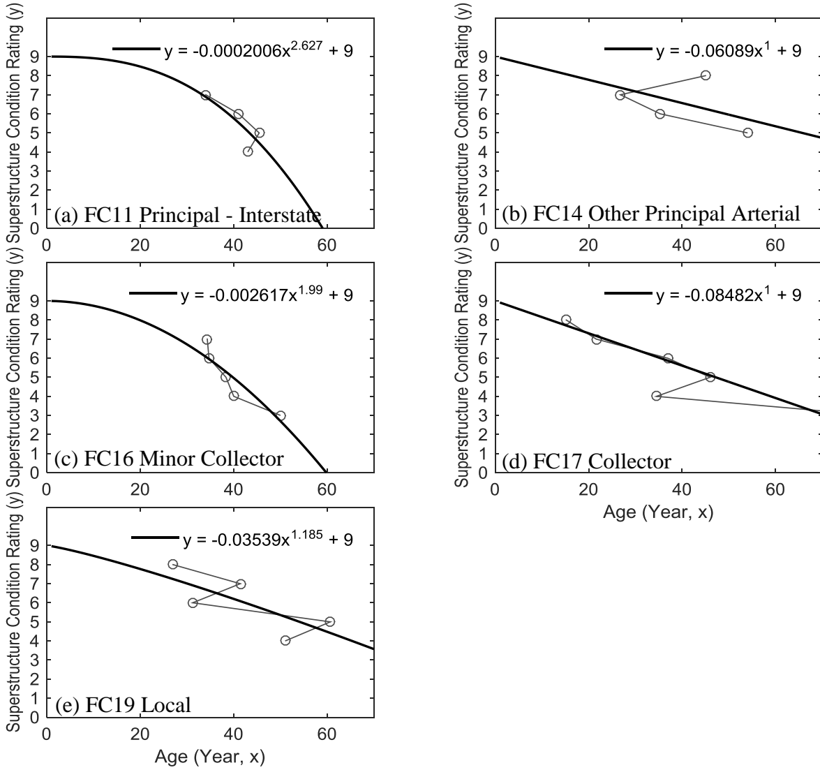
Figure 28. Graph. Deterioration models for Functional Classification of Inventory Route
