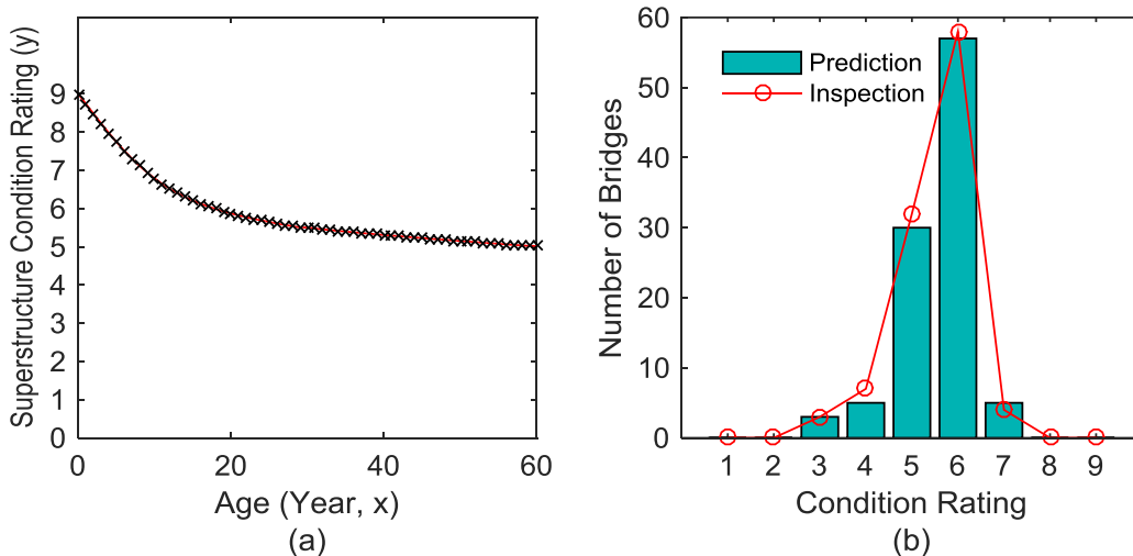
Figure 65. Graph. (a) Deterioration model and (b) comparison between prediction and inspection result in terms of number of bridges versus condition rating for DST6 (Corrugated Steel) and BRW2 (5 – 10 m, 16.4– 32.8 ft) bridges
