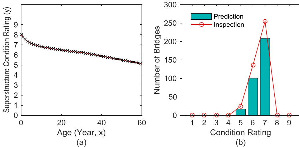
Figure 73. Graph. (a) Deterioration model and (b) comparison between prediction and inspection result in terms of number of bridges versus condition rating for WS3 (Latex Concrete/Similar) and DL6 (MS 18+Mod) bridges
