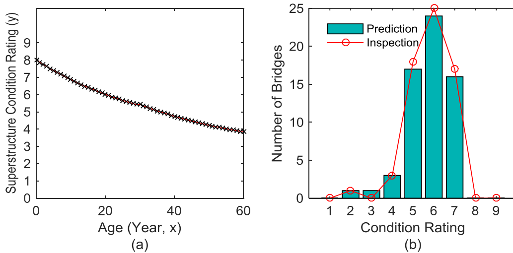
Figure 57. Graph. (a) Deterioration model and (b) comparison between prediction and inspection result in terms of number of bridges versus condition rating for WS0 (None) and SL3 – SL5 (100 m ~) bridges
