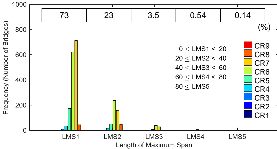
Figure 29. Chart. Distribution for Length of Maximum Span
