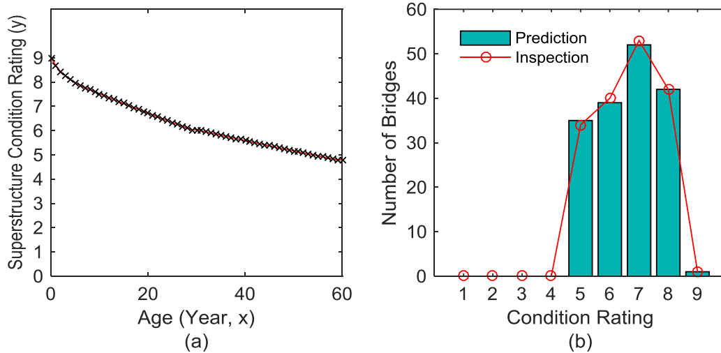
Figure 63. Graph. (a) Deterioration model and (b) comparison between prediction and inspection result in terms of number of bridges versus condition rating for DST2 (Concrete Precast Panels) and BRW2 (5 – 10 m, 16.4– 32.8 ft) bridges
