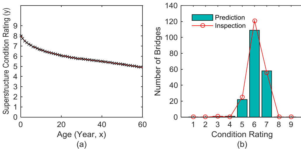
Figure 76. Graph. (a) Deterioration model and (b) comparison between prediction and inspection result in terms of number of bridges versus condition rating for WS6 (Bituminous) and DL6 (MS 18+Mod) bridges
