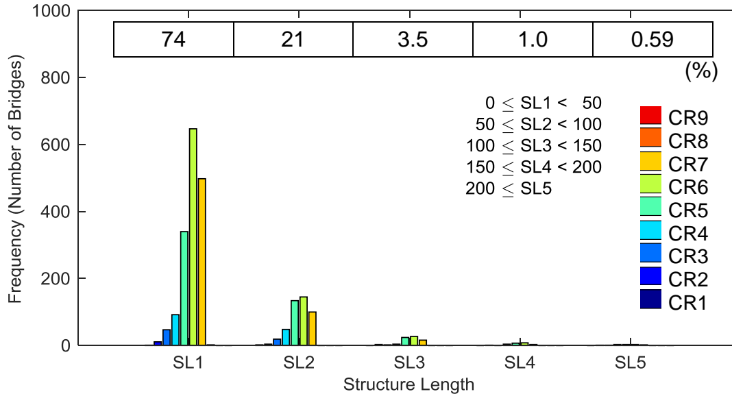
Figure 13. Chart. Distribution for Structure Length
