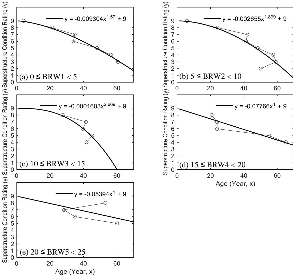
Figure 25. Graph. Deterioration models for Bridge Roadway Width (Curb to Curb)
