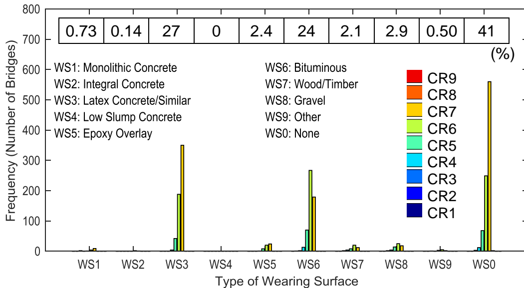
Figure 33. Chart. Distribution for Type of Wearing Surface
