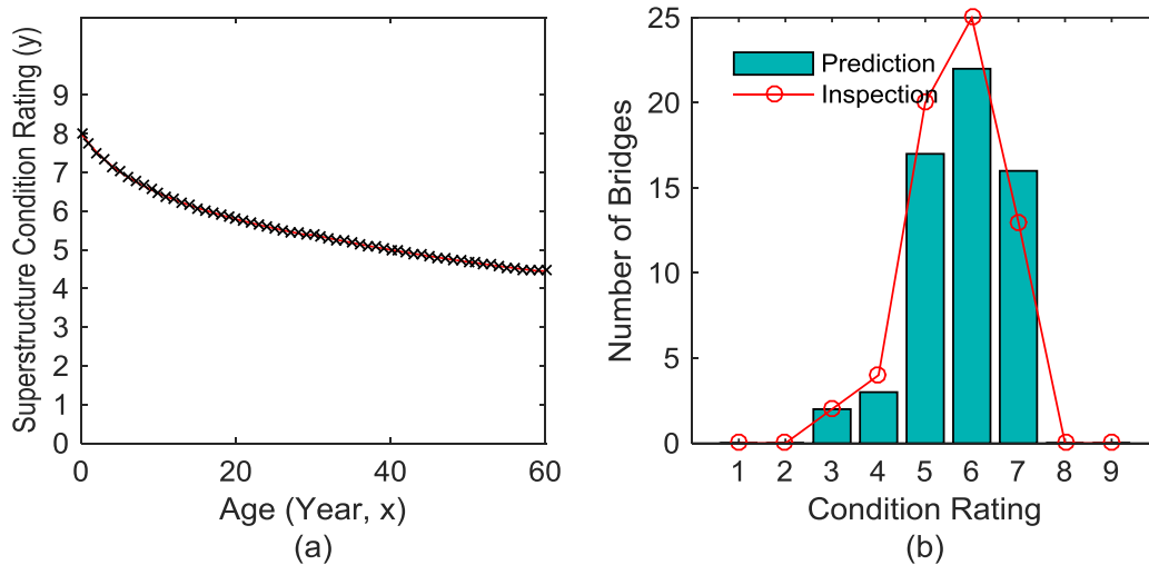
Figure 79. Graph. (a) Deterioration model and (b) comparison between prediction and inspection result in terms of number of bridges versus condition rating for WS8 (Gravel) and DL0 (Other/Unknown) bridges
