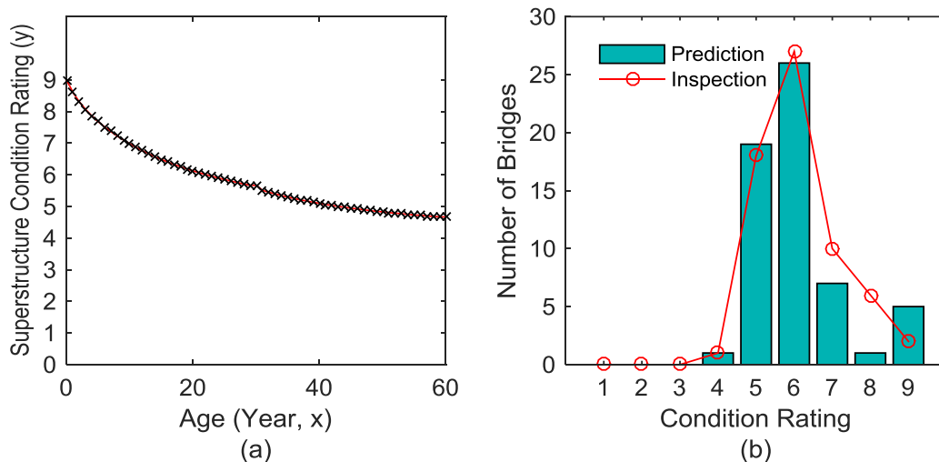
Figure 64. Graph. (a) Deterioration model and (b) comparison between prediction and inspection result in terms of number of bridges versus condition rating for DST6 (Corrugated Steel) and BRW1 (0 – 5 m, 0– 16.4 ft)bridges
