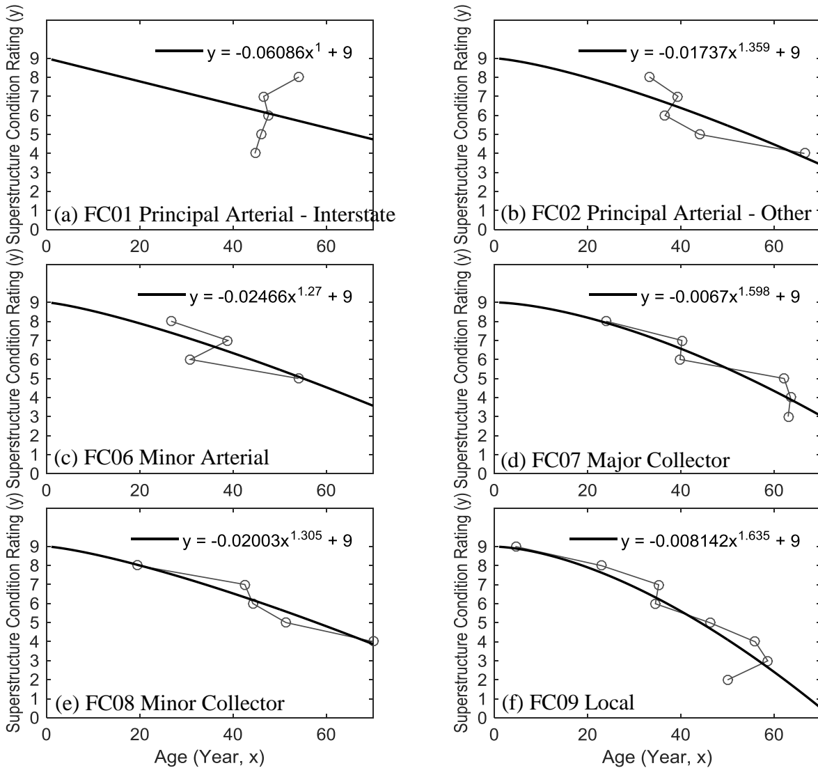
Figure 27. Graph. Deterioration models for Functional Classification of Inventory Route
