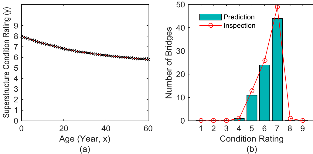
Figure 87. Graph. (a) Deterioration model and (b) comparison between prediction and inspection result in terms of number of bridges versus condition rating for WS0 (None) and DL1 - DL4 (M 9 - M 18) bridges
