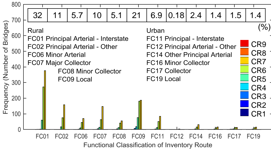
Figure 39. Chart. Distribution for Functional Classification of Inventory Route
