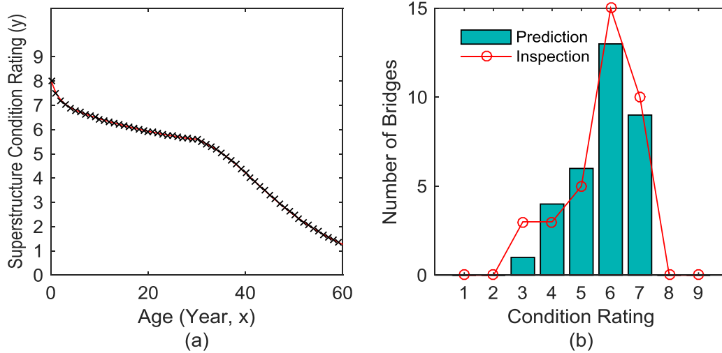
Figure 56. Graph. (a) Deterioration model and (b) comparison between prediction and inspection result in terms of number of bridges versus condition rating for WS5 (Epoxy Overlay) and SL1 – SL5 bridges
