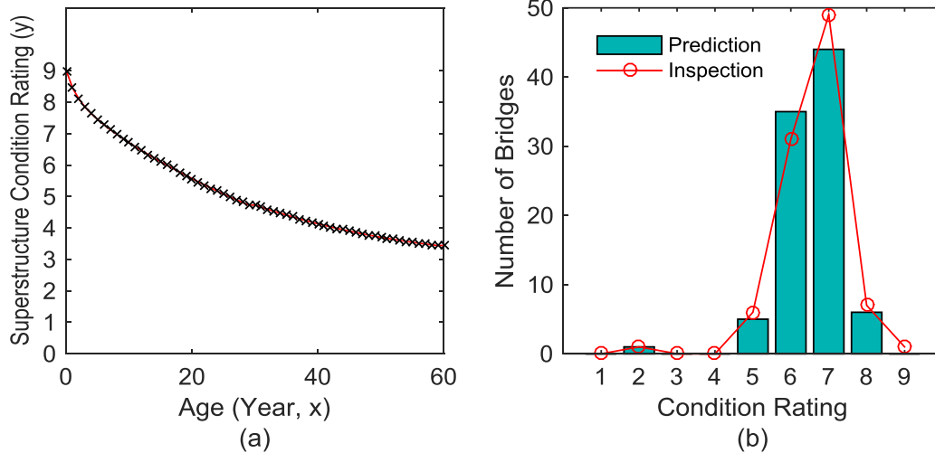
Figure 52. Graph. (a) Deterioration model and (b) comparison between prediction and inspection result in terms of number of bridges versus condition rating for WS7 (Wood/Timber) and SL1 (0 – 50 m) bridges
