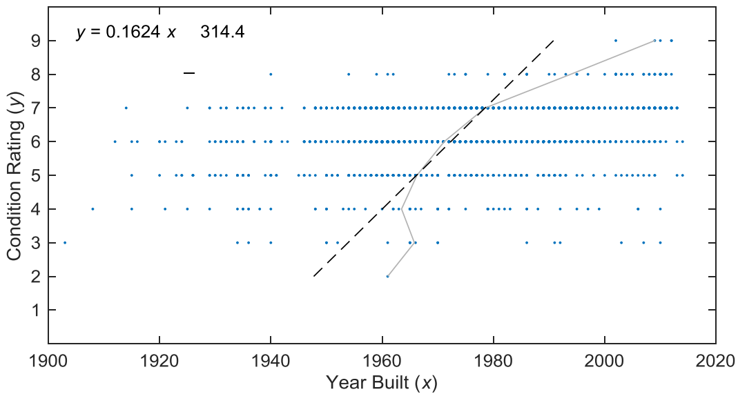
Figure 31. Graph. Condition rating versus year built for bridge substructure at year 2014
