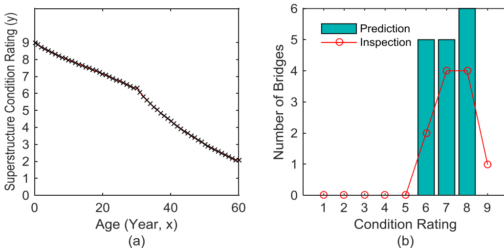
Figure 70. Graph. (a) Deterioration model and (b) comparison between prediction and inspection result in terms of number of bridges versus condition rating for rest bridges
