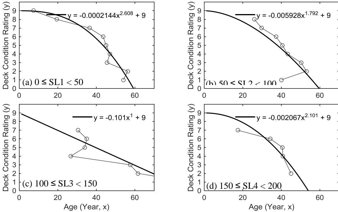
Figure 14. Graph. Deterioration models for Structure Length
