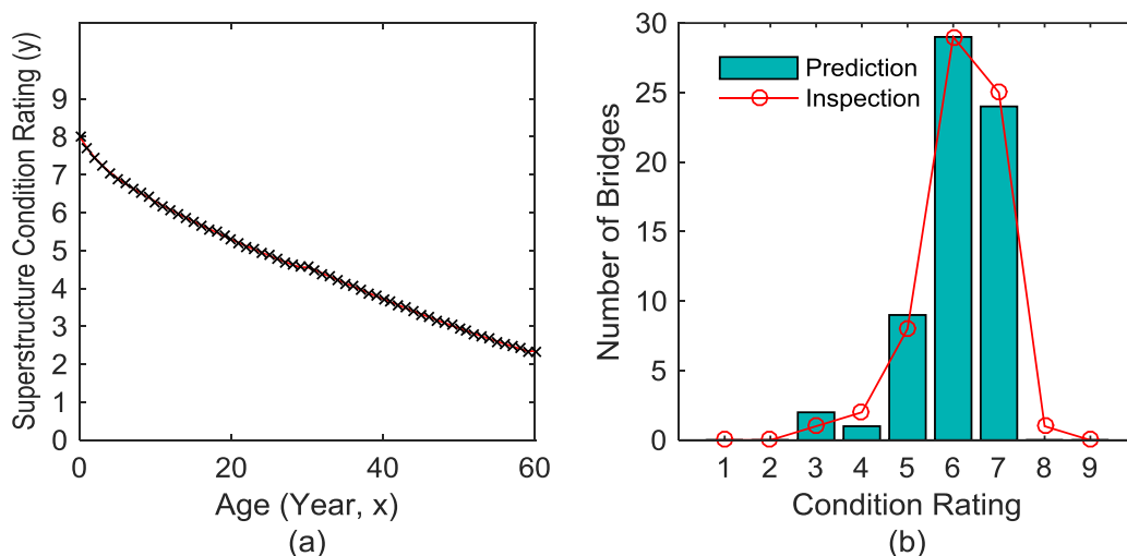
Figure 78. Graph. (a) Deterioration model and (b) comparison between prediction and inspection result in terms of number of bridges versus condition rating for WS7 (Wood/Timber) and DL0 (Other/Unknown) bridges
