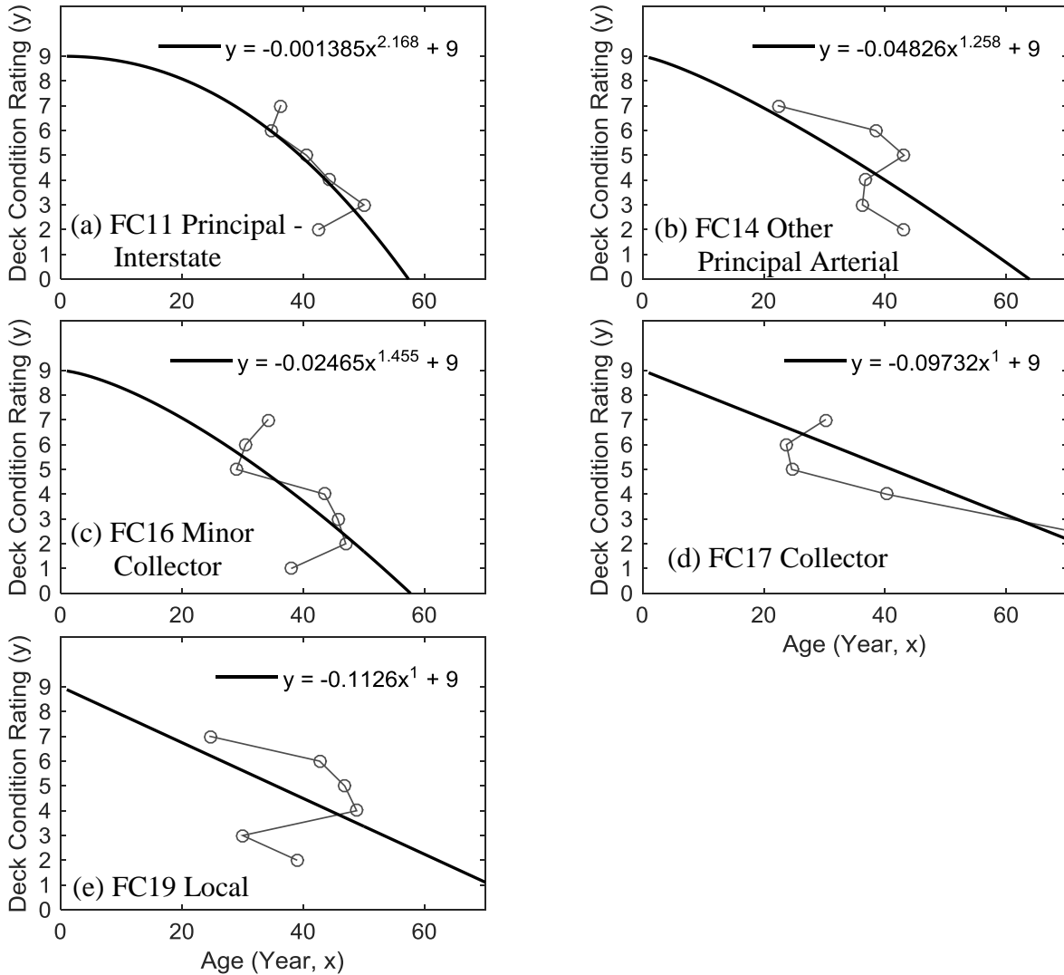
Figure 17. Graph. Deterioration models for Functional Classification of Inventory Route belonging to the urban category
