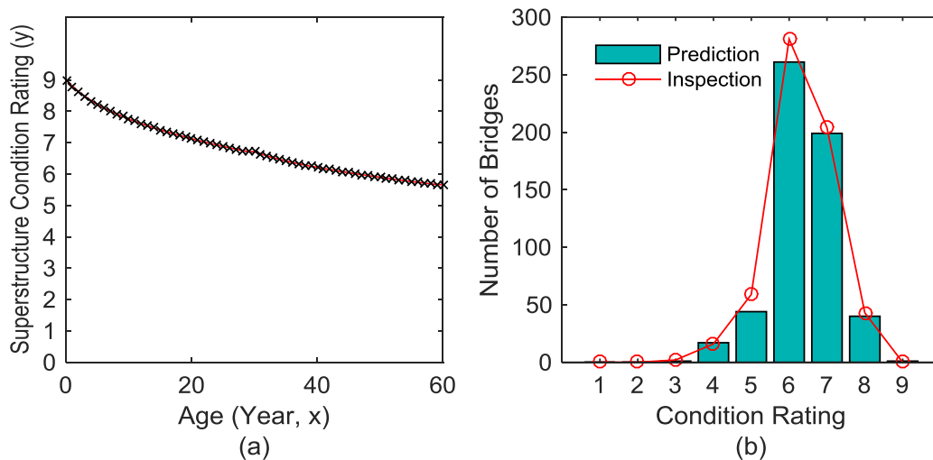
Figure 60. Graph. (a) Deterioration model and (b) comparison between prediction and inspection result in terms of number of bridges versus condition rating for DST1 (Concrete Cast-in-Place) and BRW2 (5 – 10 m, 16.4– 32.8 ft) bridges
