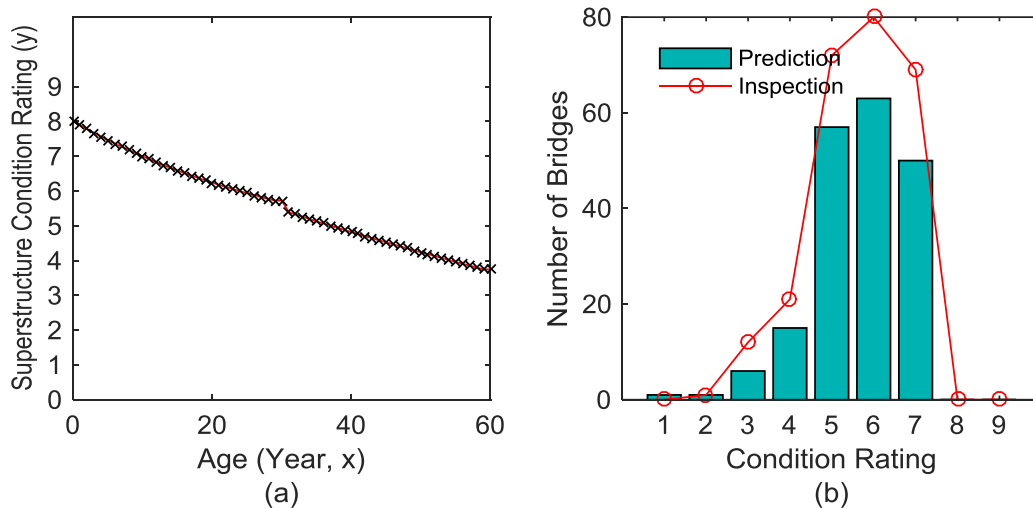
Figure 55. Graph. (a) Deterioration model and (b) comparison between prediction and inspection result in terms of number of bridges versus condition rating for WS0 (None) and SL2 (50 – 100 m) bridges
