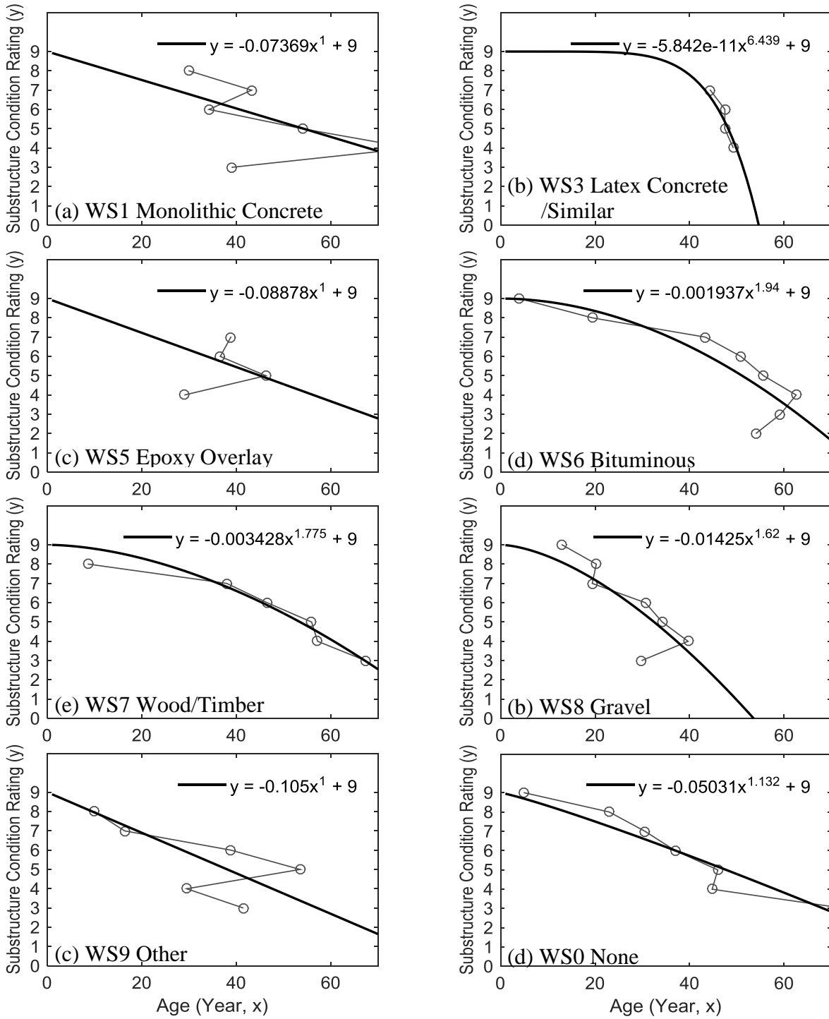
Figure 34. Graph. Deterioration models for Wearing Surface
