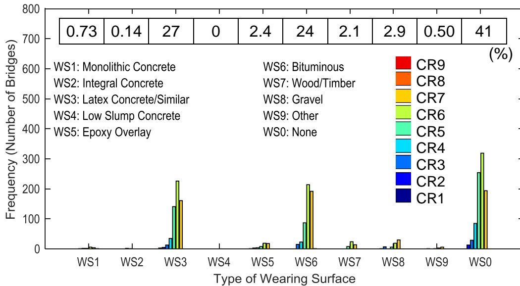
Figure 11. Chart. Distribution for Type of Wearing Surface
