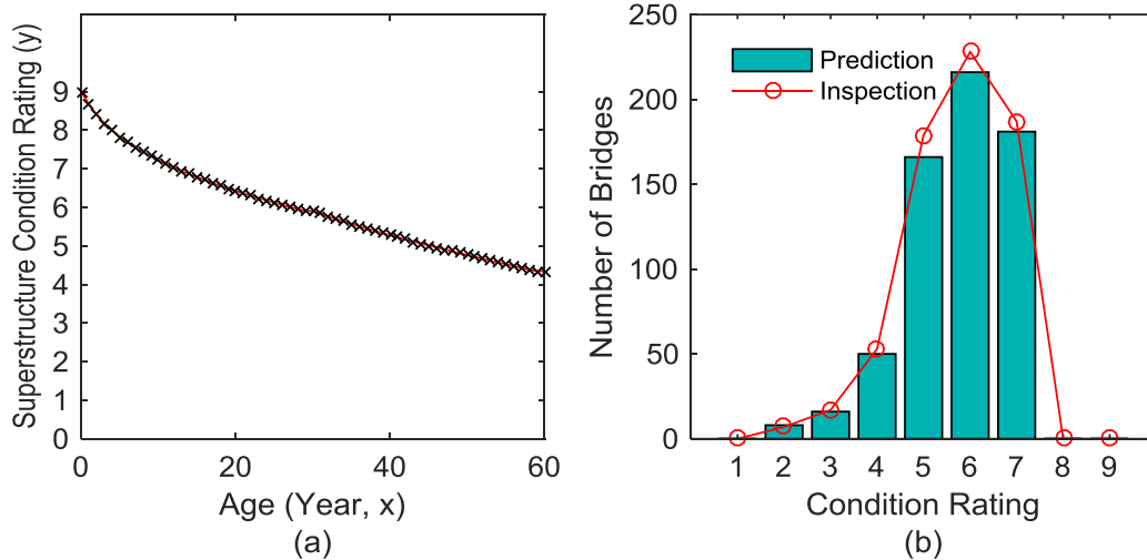
Figure 54. Graph. (a) Deterioration model and (b) comparison between prediction and inspection result in terms of number of bridges versus condition rating for WS0 (None) and SL1 (0 – 50 m) bridges
