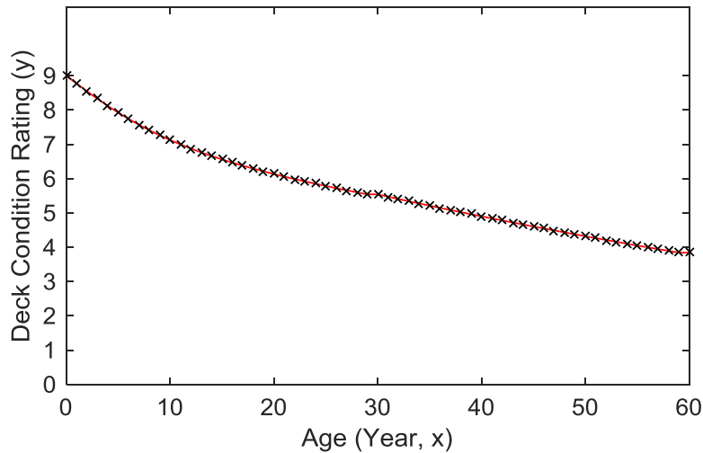
Figure 48. Graph. Deterioration model for deck element
