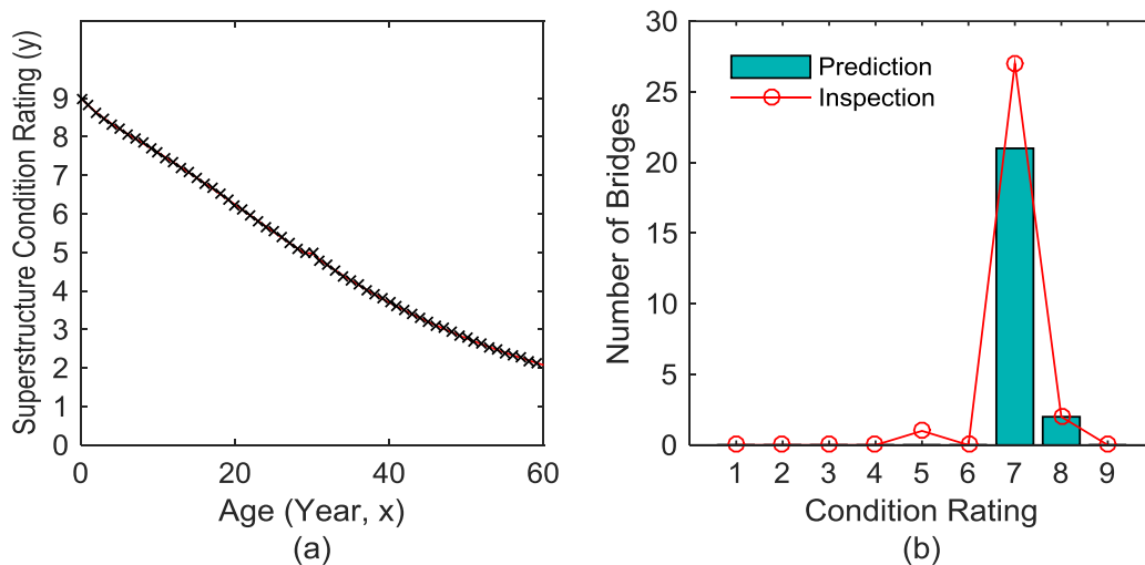
Figure 62. Graph. (a) Deterioration model and (b) comparison between prediction and inspection result in terms of number of bridges versus condition rating for DST1 (Concrete Cast-in-Place) and BRW4 (15 – 20 m, 49.2 – 65.6 ft) bridges
