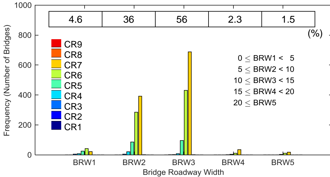
Figure 37. Chart. Distribution for Bridge Roadway Width (Curb to Curb)
