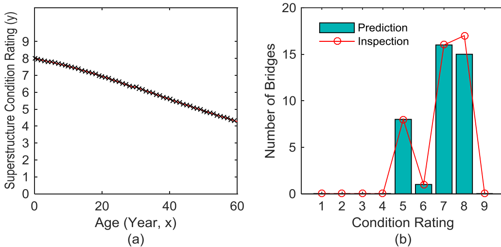
Figure 69. Graph. (a) Deterioration model and (b) comparison between prediction and inspection result in terms of number of bridges versus condition rating for DST2 (Concrete Precast Panels) and BRW1, BRW3 – BRW5 bridges
