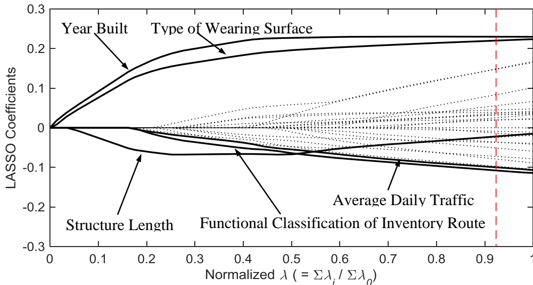
Figure 6. Graph. Solution path for deck condition ratings by LASSO
