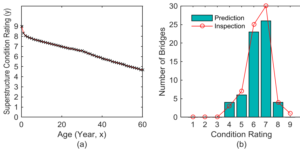
Figure 85. Graph. (a) Deterioration model and (b) comparison between prediction and inspection result in terms of number of bridges versus condition rating for WS6 (Bituminous) and DL1 (M 9), DL3 (MS 13.5), DL4 (M 18), and DL9 (MS 22.5) bridges
