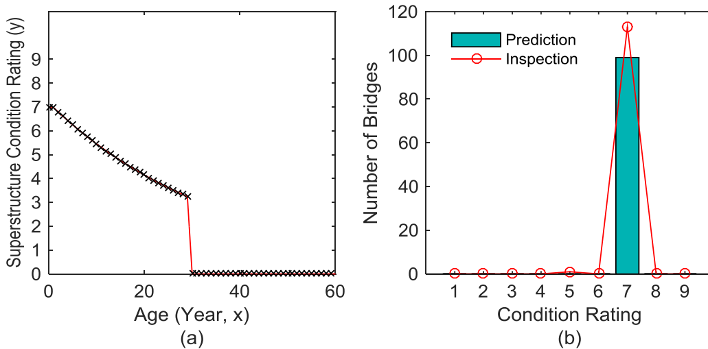
Figure 82. Graph. (a) Deterioration model and (b) comparison between prediction and inspection result in terms of number of bridges versus condition rating for WS0 (None) and DL9 (MS 22.5) bridges
