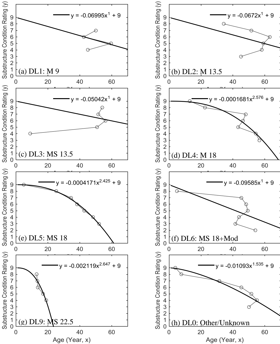
Figure 36. Graph. Deterioration models for Design Load
