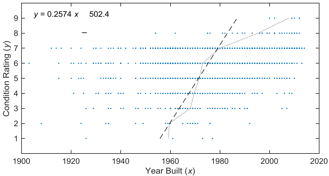
Figure 9. Graph. Condition rating versus year built for bridge deck at year 2014
