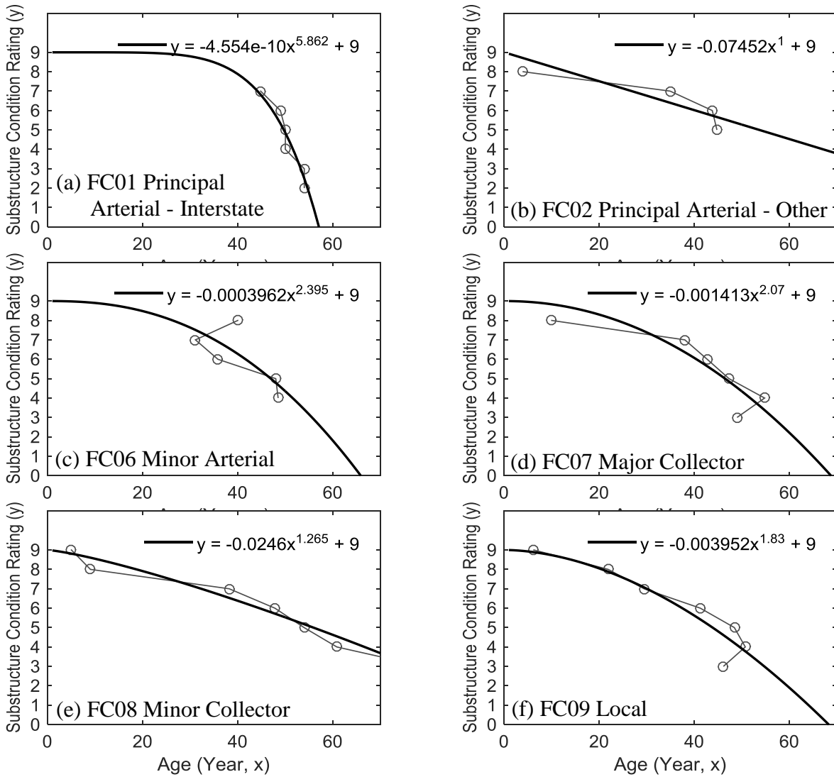
Figure 40. Graph. Deterioration models for Functional Classification of Inventory Route
