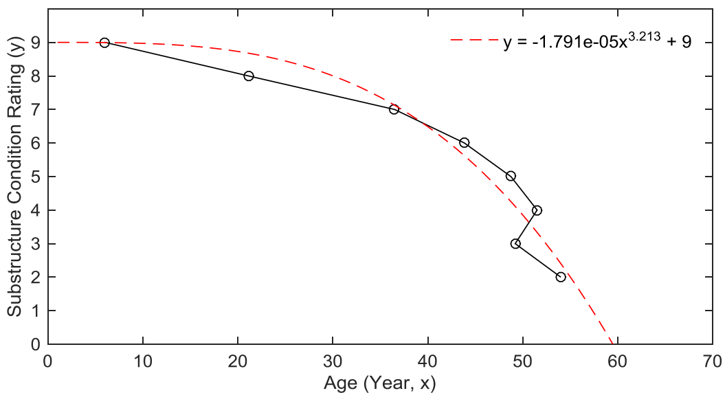
Figure 32. Graph. Deterioration model for substructure elements
