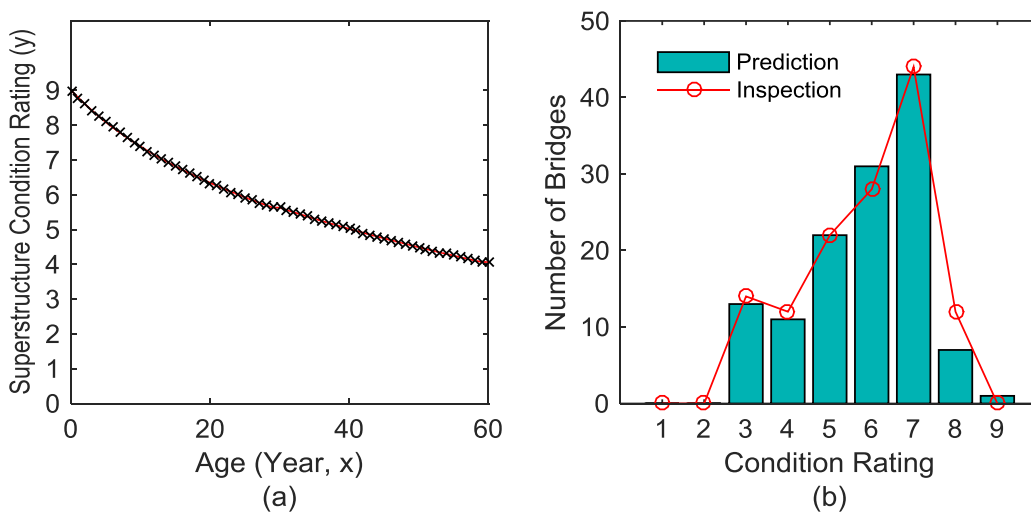
Figure 66. Graph. (a) Deterioration model and (b) comparison between prediction and inspection result in terms of number of bridges versus condition rating for DST8 (Wood/Timber) and BRW1 (0 – 5 m, 0 ft – 16.4 ft) bridges
