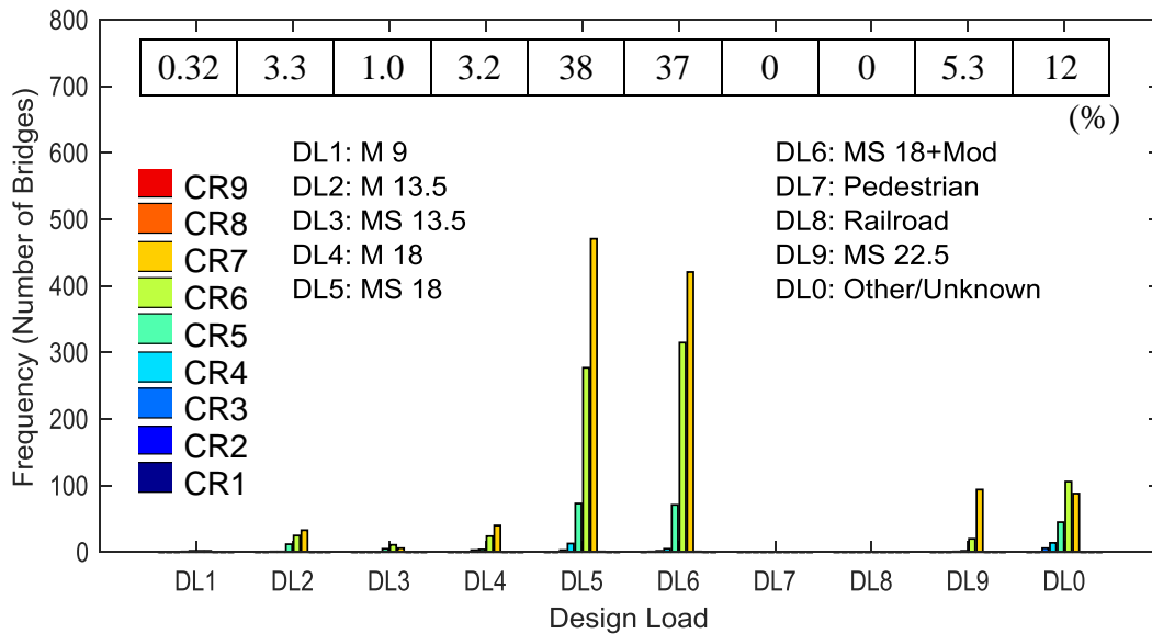
Figure 35. Chart. Distribution for Design Load
