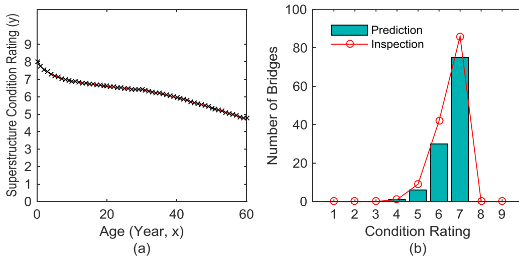
Figure 72. Graph. (a) Deterioration model and (b) comparison between prediction and inspection result in terms of number of bridges versus condition rating for WS3 (Latex Concrete/Similar) and DL5 (MS 18) bridges
