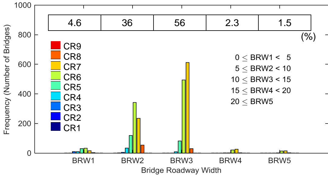
Figure 24. Chart. Distribution for Bridge Roadway Width (Curb to Curb)
