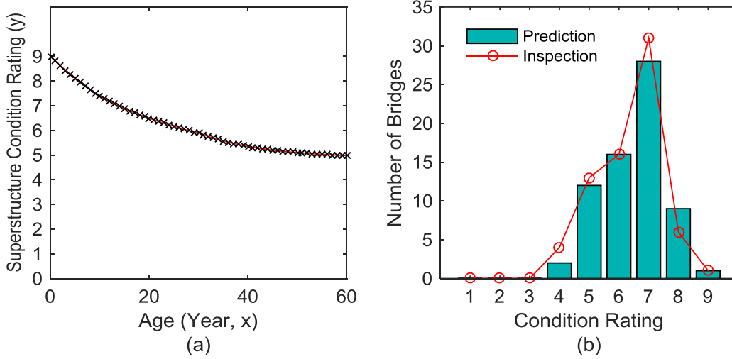
Figure 86. Graph. (a) Deterioration model and (b) comparison between prediction and inspection result in terms of number of bridges versus condition rating for WS8 (Gravel) and DL1 – DL9 (all except DL0) bridges
