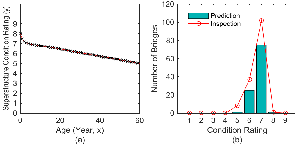
Figure 81. Graph. (a) Deterioration model and (b) comparison between prediction and inspection result in terms of number of bridges versus condition rating for WS0 (None) and DL6 (MS 18+Mod) bridges
