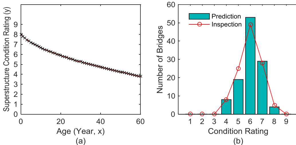
Figure 77. Graph. (a) Deterioration model and (b) comparison between prediction and inspection result in terms of number of bridges versus condition rating for WS6 (Bituminous) and DL0 (Other/Unknown) bridges
