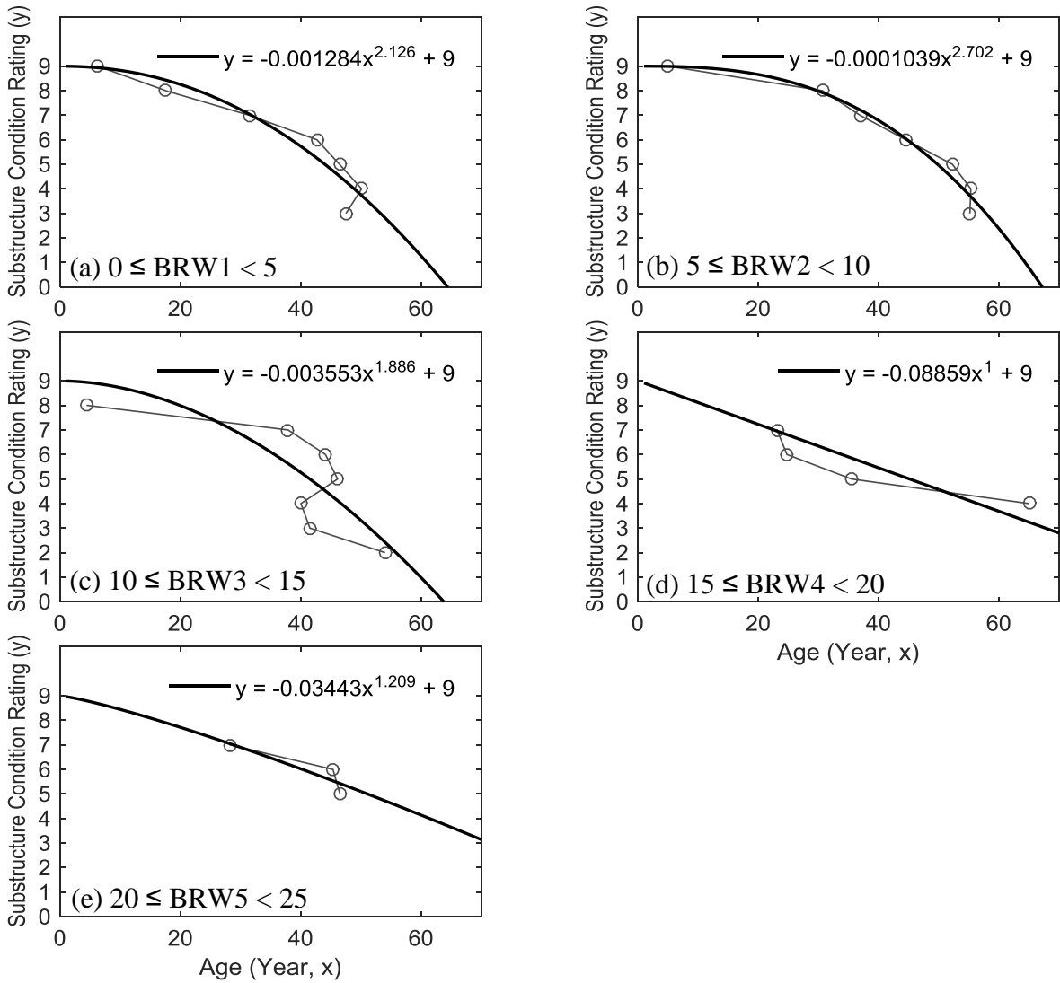
Figure 38. Graph. Deterioration models for Bridge Roadway Width (Curb to Curb)
