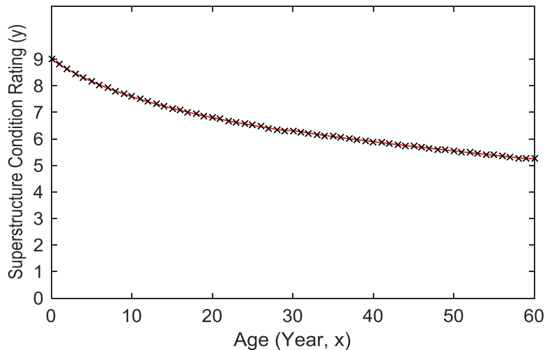
Figure 59. Graph. Deterioration model for superstructure element
