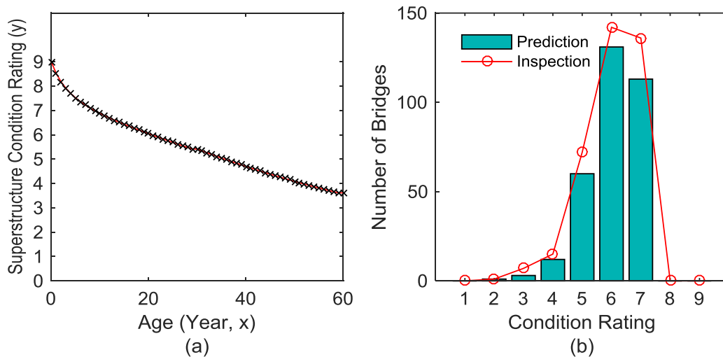
Figure 49. Graph. (a) Deterioration model and (b) comparison between prediction and inspection result in terms of number of bridges versus condition rating for WS3 (Latex Concrete/Similar) and SL1 (0 – 50 m) bridges
