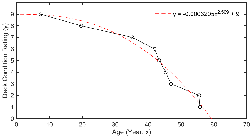
Figure 10. Graph. General deterioration model for deck elements
