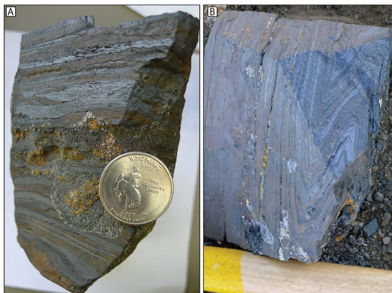
Figure 6. A and B) Banded iron formation from south of the Atlantic City Iron Mine (sample 20140925WS-A). Both images show metallic banding and recumbent folding.
