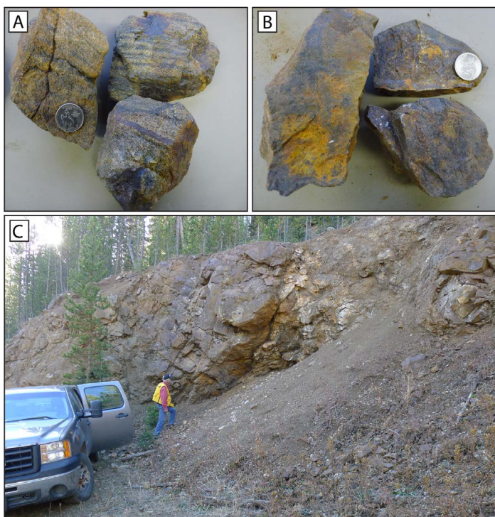
Figure 17. Wildcat Creek deposit (sample 20141016WS-A) with A) magnetite banding, possibly a metamorphosed BIF, B) a range of limonite and hematite staining and metallic sheen, and C) a view of the outcrop and fault zone.
