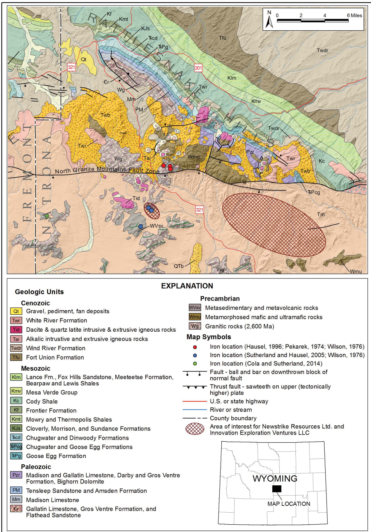
Figure 11. Geology of the Rattlesnake Hills-Granite Mountains area. BIF is found in metamorphosed Precambrian units. The area of iron resources being investigated by Newstrike Resources Ltd. and Innovation Exploration Ventures, LLC is emphasized. Map modified from Love and Christiansen (1985, 2014).
