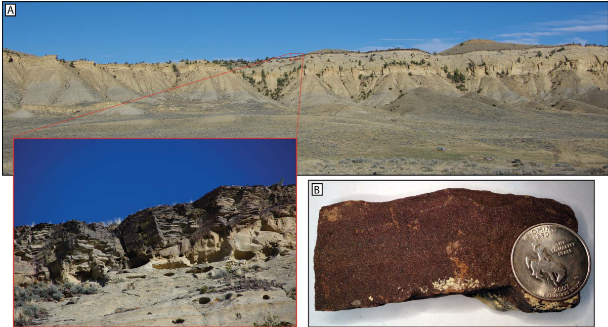
Figure 32. A) Panorama of the Grass Creek North black sandstone deposit and location of sample 20141015WS-D. The dark, magnetite-rich layer can be seen at the top with varying thickness. The inset photo shows the layer in more detail. B) Close up of the black sandstone with varying color and slight layering.
