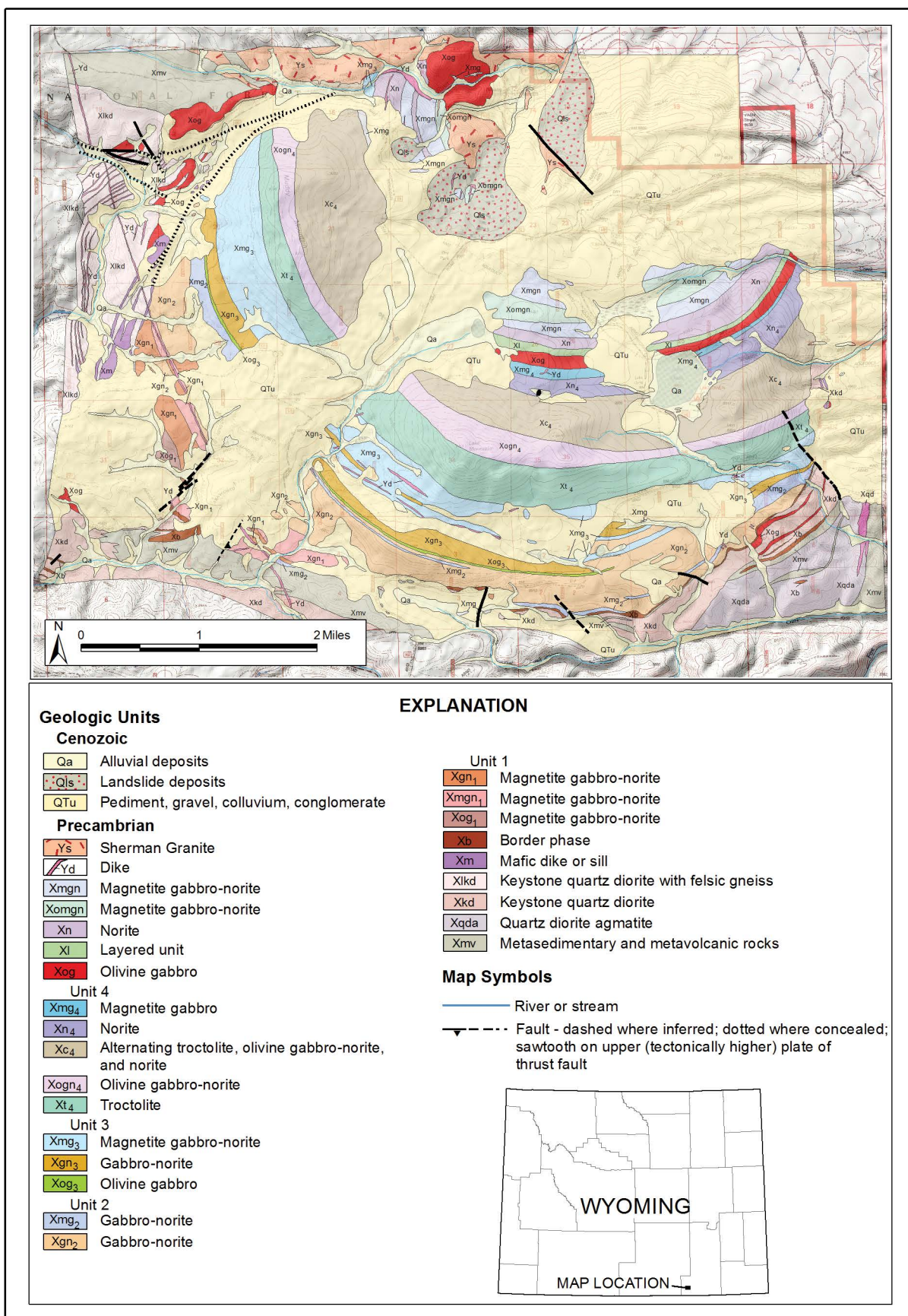
Figure 16. Geology of the Lake Owen complex in the Medicine Bow Mountains. The Lake Owen mafic complex consists of alternating layers of olivine and magnetite-rich gabbro and norite. Detailed unit descriptions can be found in text. Modified from an unpublished map by Houston and others.
