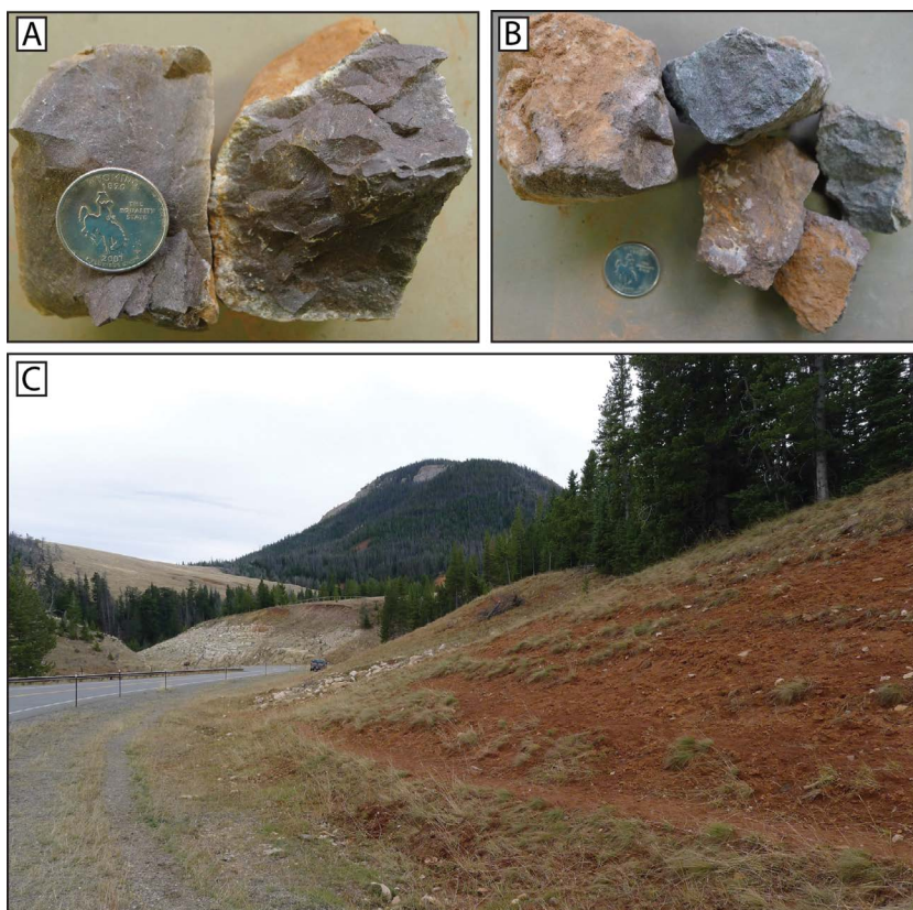
Figure 22. Hematite-rich Amsden Formation occurs near Pat O'Hara Mountain. A) Concretionary hematite with a maroon hue. B) Concretions with bluish-black color and a slight metallic luster (sample 20141015WS-B). C) The outcrop of Amsden Formation with a southeast view toward Pat O'Hara Mountain.
