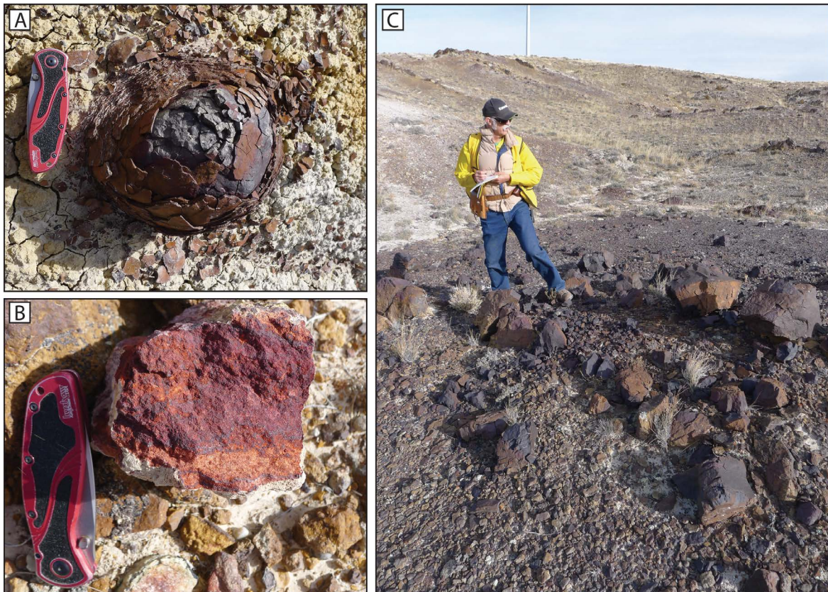
Figure 29. Iron deposits at the Deacon's Prayer Group claim. A) Concentric, cannonball-type iron concretion. B) Hematite-rich sandstone with thin metallic banding (sample 20141023WS-D). C) Geologist Wayne Sutherland investigates a concretionary iron layer (sample 20141023WS-B).
