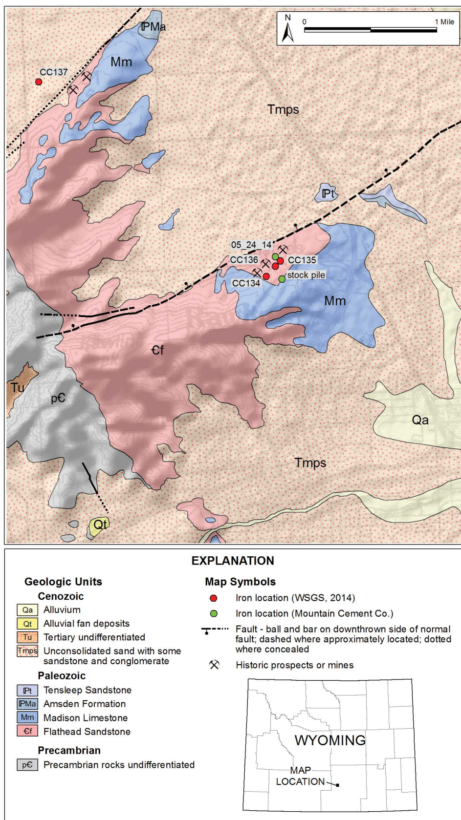
Figure 19. Geology of the Rawlins area where hematite deposits occur just north of the city. Some samples reside within the historic Rawlins Red mine area. Map modified from McLaughlin and Fruhwirth (2008).
