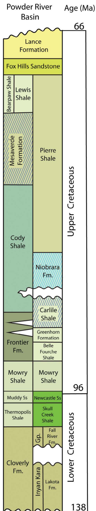
Figure 26. Stratigraphic column showing the relationships of Cretaceous units in the Powder River Basin in northeast Wyoming. Modified from Love and others (1993), and colors updated to correlate with Love and Christiansen (1985, 2014).
