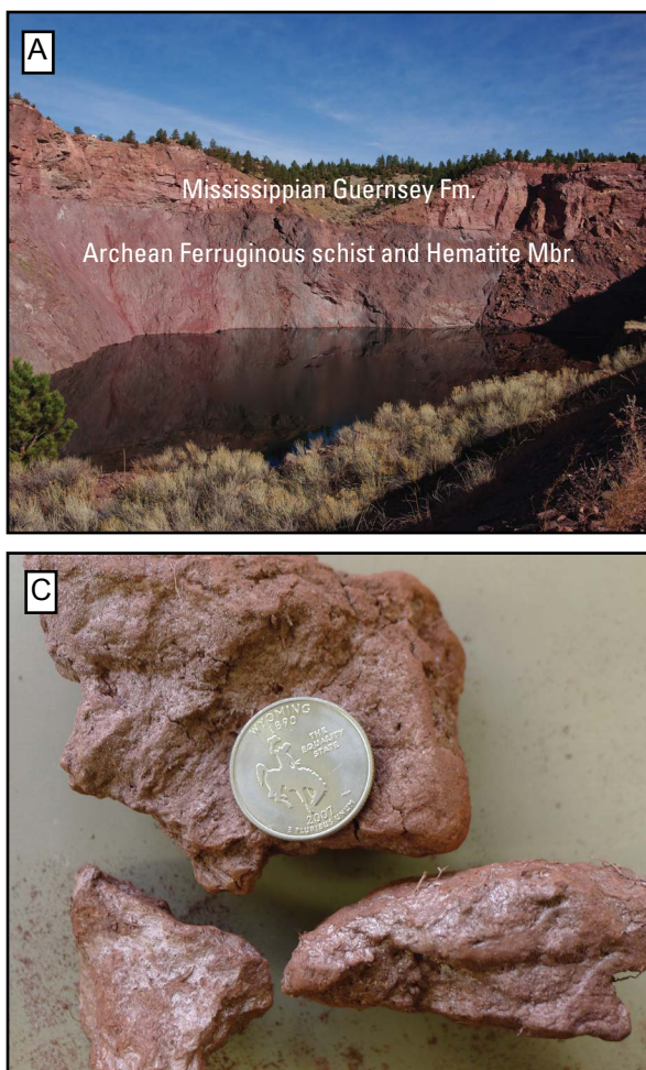
Figure 8. Images from the Sunrise Mine near Hartville, Wyoming. A) The main pit now filled with water. The Mississippian Guernsey Formation is the cap rock overlying the Archean Ferruginous schist and Hematite members. B) Red ochre accompanied by greenish opaline chert sampled from an archeological site near the main pit. C.) Red, ultra-fine pond tailings (sample 20140926WS-C) held together by clay.
