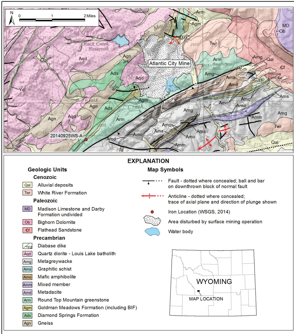
Figure 5. Sample location and geology of the southern Wind River Mountains near the Atlantic City Iron Mine. The sampled BIF occurs in the Goldman Meadows Formation. Map modified from Johnson and Sutherland (2009).
