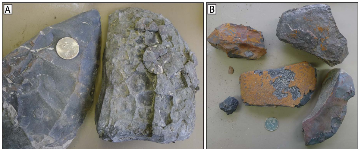
Figure 27. Iron concretions (samples 20141014WS-A & B) collected from the Belle Fourche Formation in northeastern Wyoming. A) “Alligator skin” texture and B) a variety of shapes, textures, and coloration of concretions.
