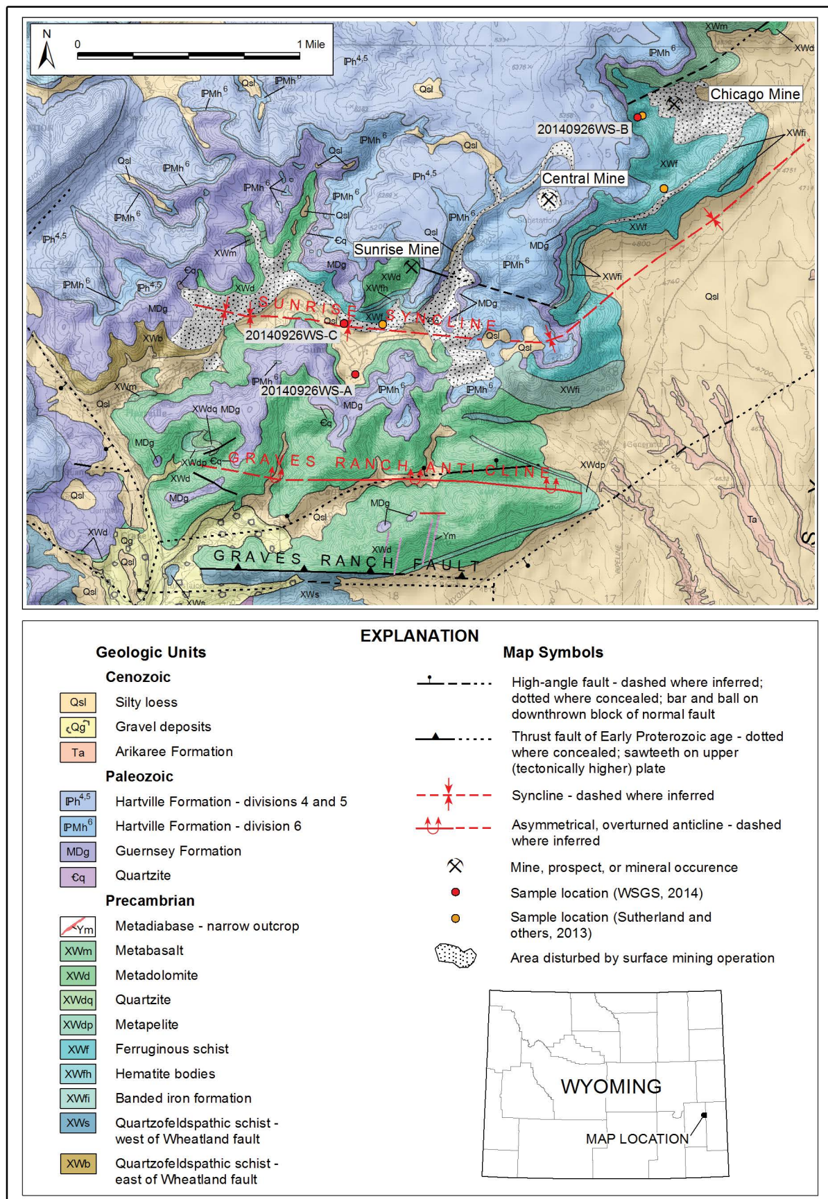
Figure 7. Geology of the Hartville Uplift area showing the Sunrise, Central, and Chicago mines along with WSGS sample locations. Map modified from Harris and others (2005).
