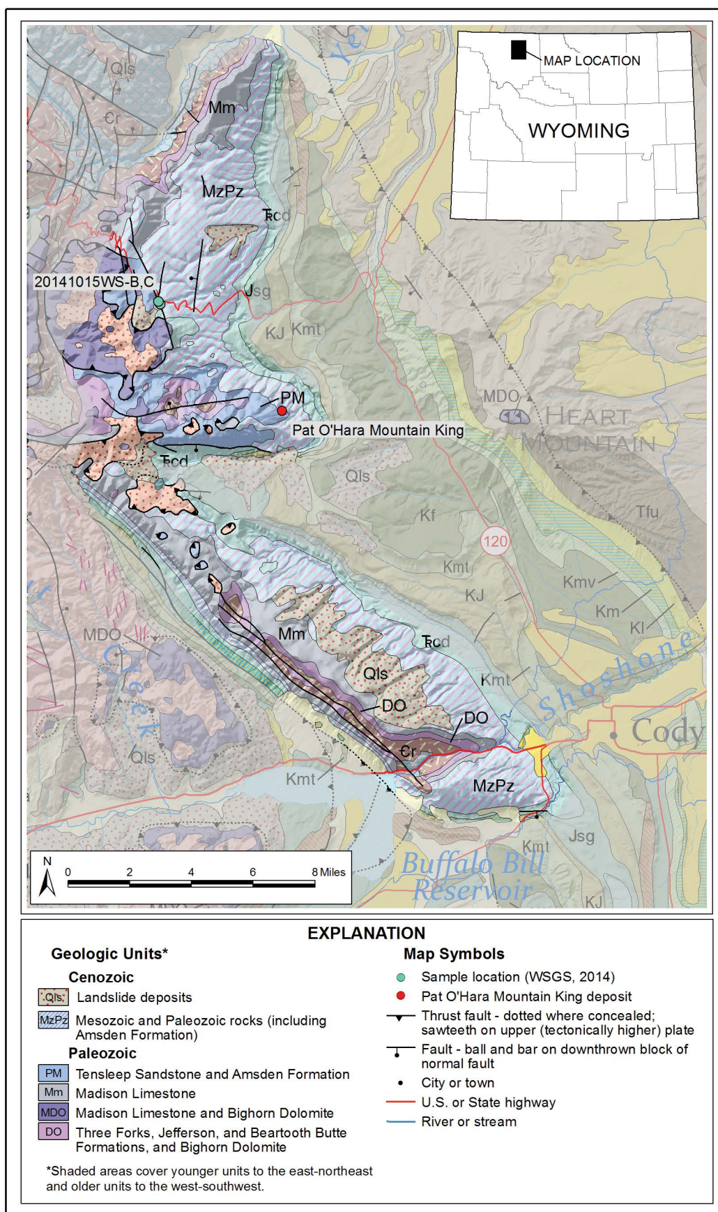
Figure 21. Geology of the eastern edge of the Absaroka Mountains near Cody, focusing on the Paleozoic formations. Iron occurs locally within the Amsden Formation. Sampling was based on potential continuity with the Pat O'Hara Mountain King deposit. Map modified from Love and Christiansen (1985, 2014).
