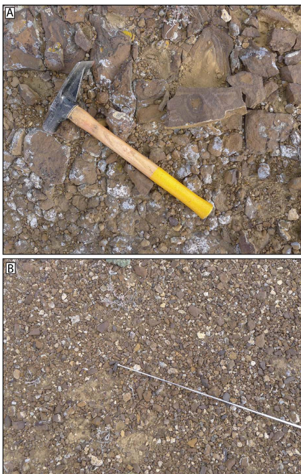
Figure 31. Lovell deposit black sandstone with A) concentric banding and differential weathering surfaces and B) magnetite pebble debris with a magnet attracted to a piece (sample 20141015WS-A).
