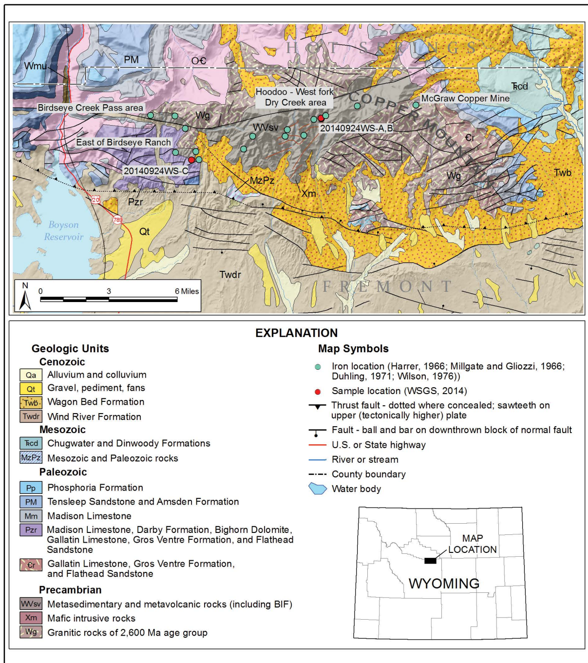
Figure 12. Geology of the Copper Mountain area. BIF occurs near the McGraw copper mine, the Hoodoo-West Fork Cry Creek area, east of Birdseye Ranch, and in the Birdseye Creek Pass area. Map modified from Love and Christiansen (1985, 2014).
