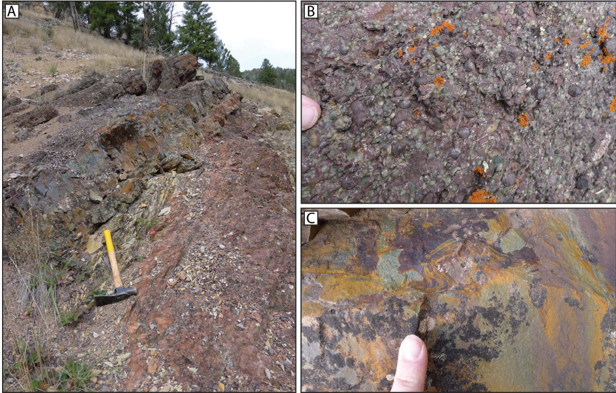
Figure 23. Sheep Creek Canyon locality in the Western Wyoming Range. A) The bottom layer is a hard, red, silty shale (sample 20141016WS-B), the middle layer is fissile, variegated shale, and the top layer a variegated pisolite (sample 20141016WS-C). B) A close up of the pisolite. C) A close up of the variegated shale.
